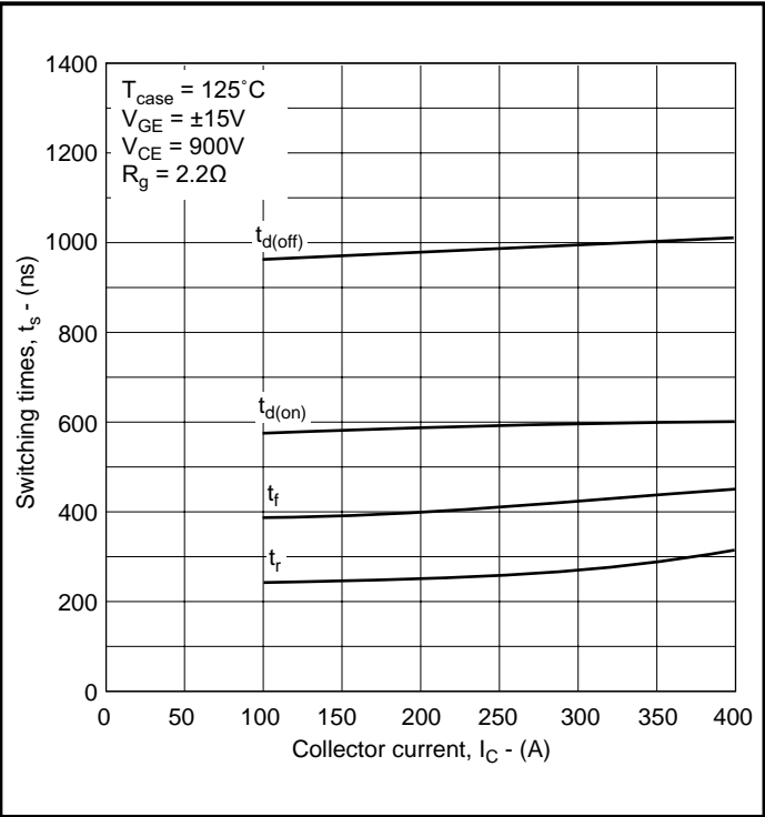
Fig. 10 Typical switching times
