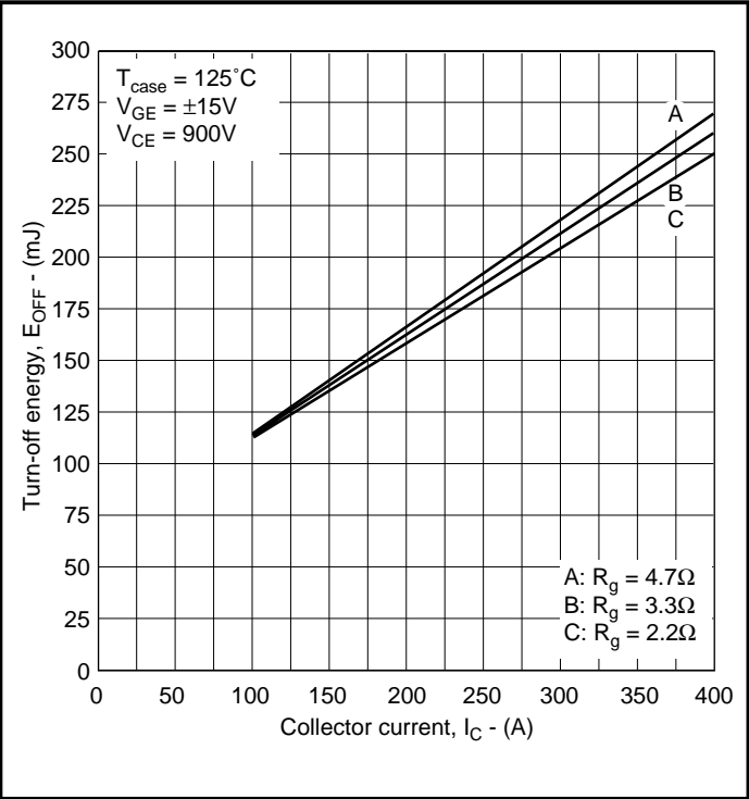
Fig. 8 Typical turn-off energy vs collector current
