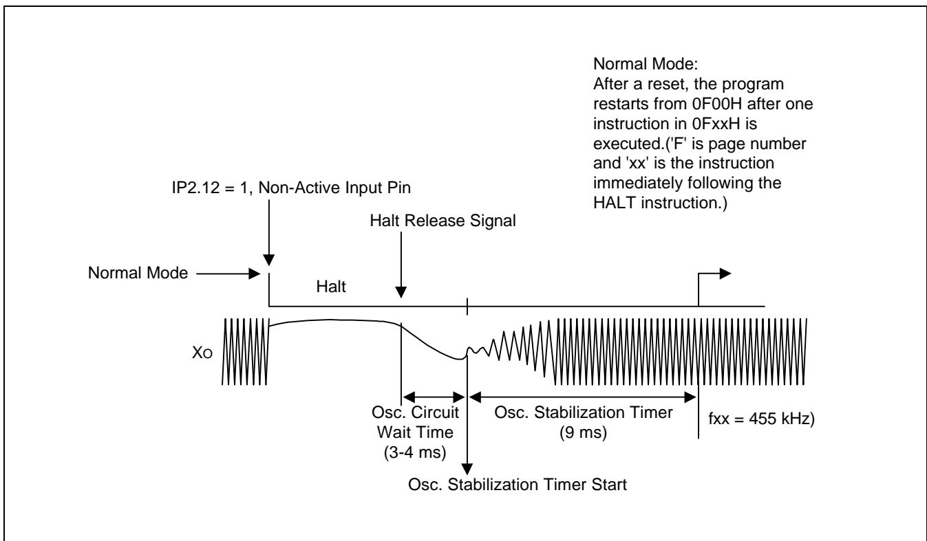
Figure 7-3. Reset Timing Diagram
