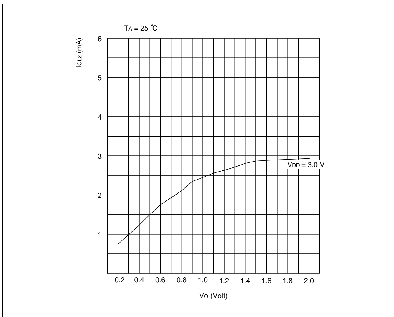
Figure 3-24. I_{OL2} vs V_O (P3.0-P3.3)
