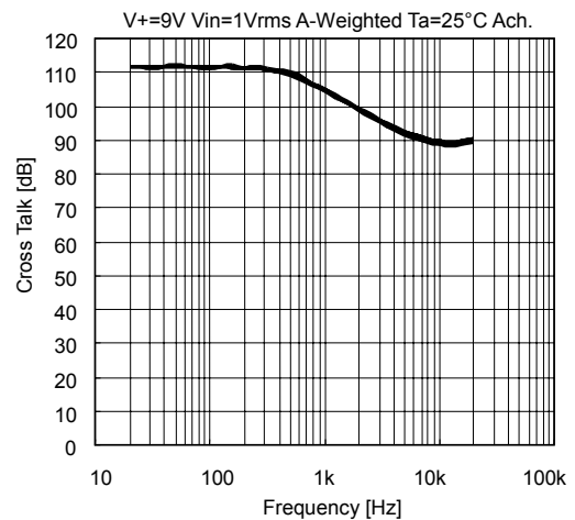
Cross Talk vs Frequency Response
