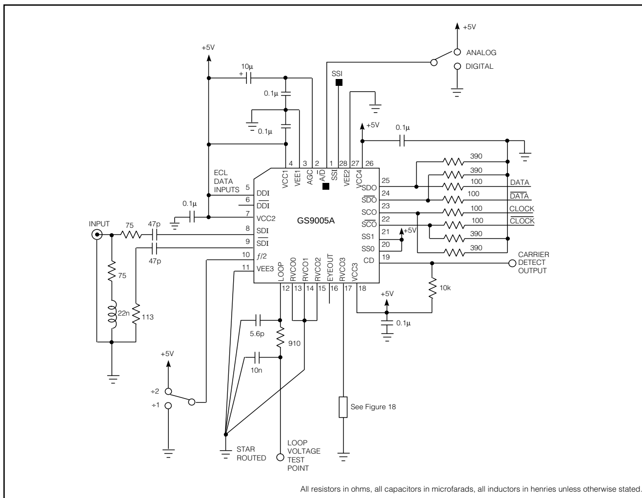
Fig.16 GS9005A Typical Test Circuit Using +5V Supply
