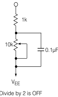
Fig. 19 Non - Temperature Compensated Resistor Values for 143 Mb/s and 177 Mb/s
