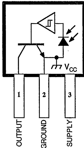
ULN3330/60/63T
