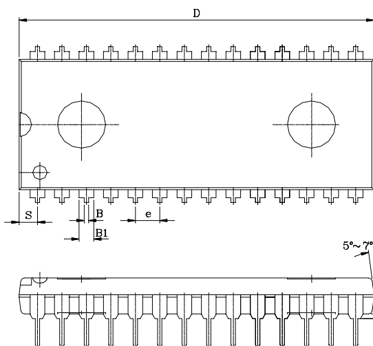
PDIP - 28
