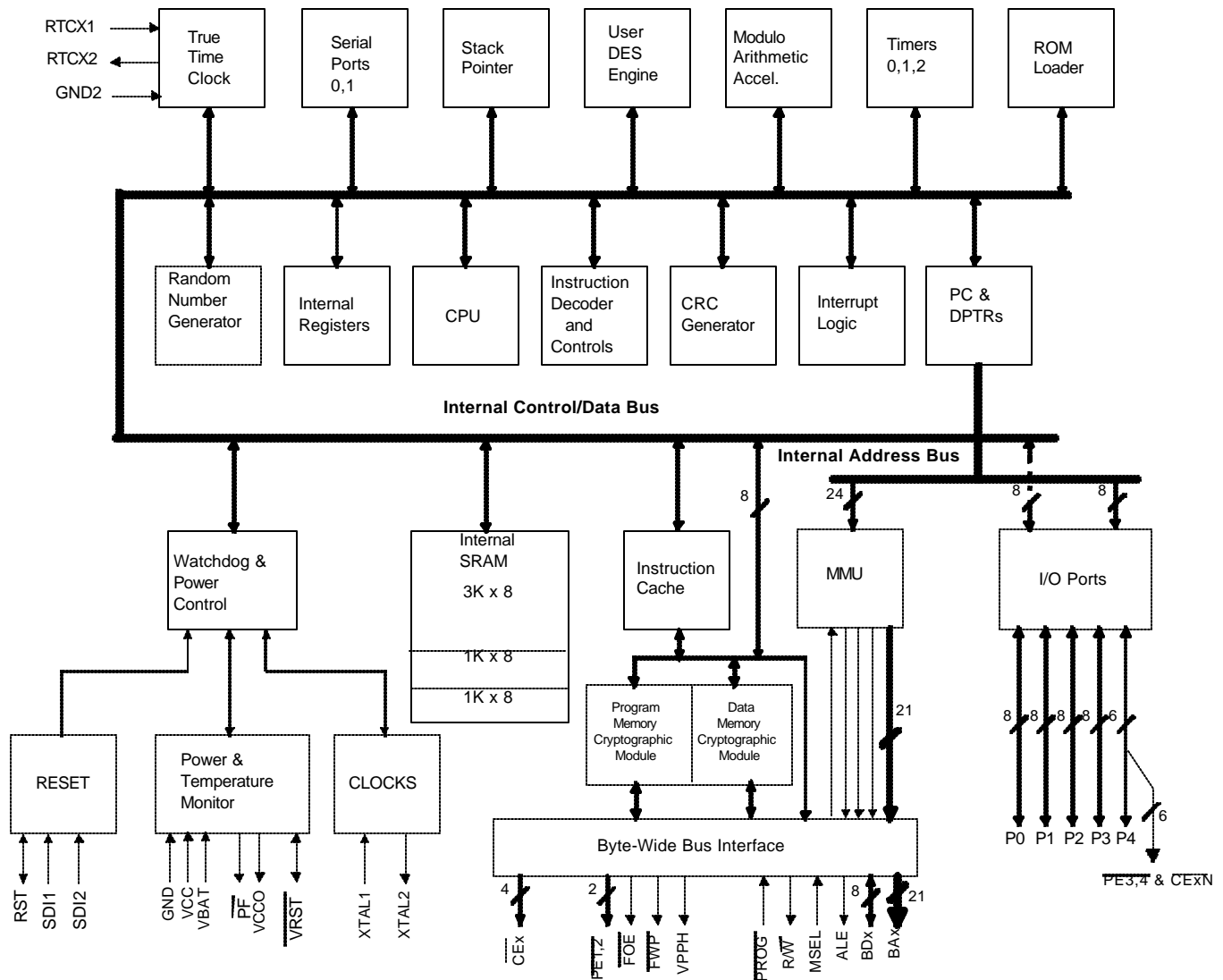
Figure 1. BLOCK DIAGRAM
