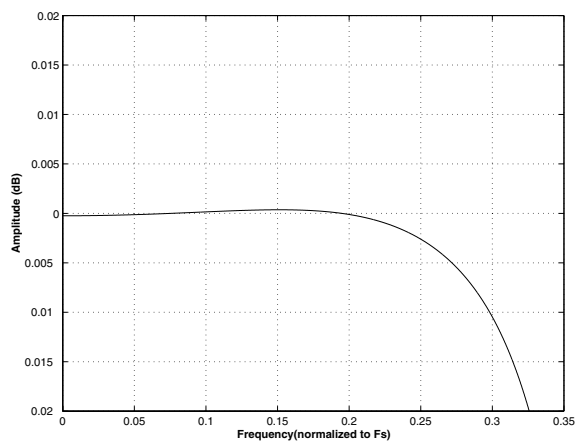
Figure 24. Double Speed (slow) Passband Ripple
