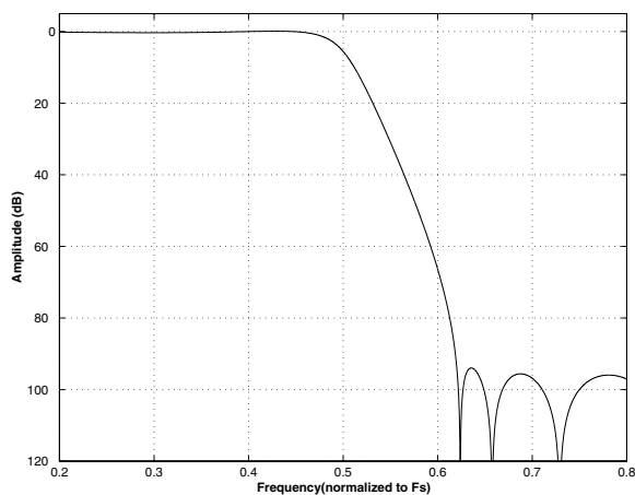
Figure 26. Quad Speed (fast) Transition Band
