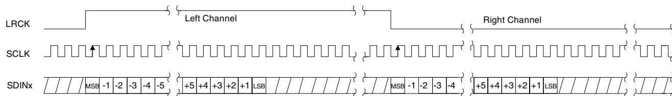
Figure 33. Format 0 - Left Justified up to 24-bit Data
