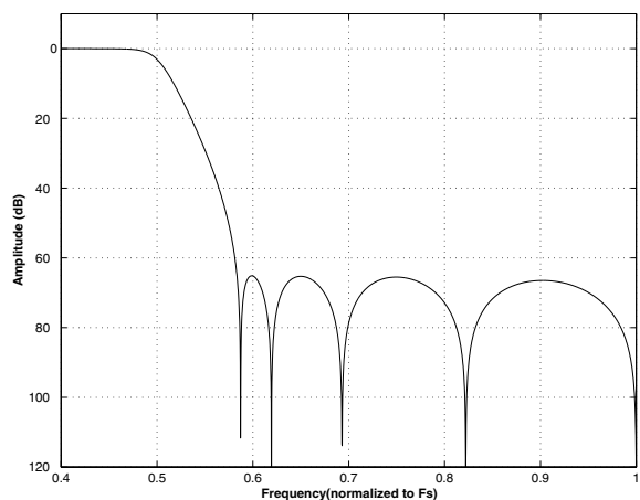
Figure 13. Single Speed (slow) Stopband Rejection
