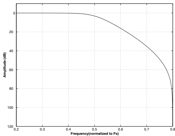
Figure 22. Double Speed (slow) Transition Band
