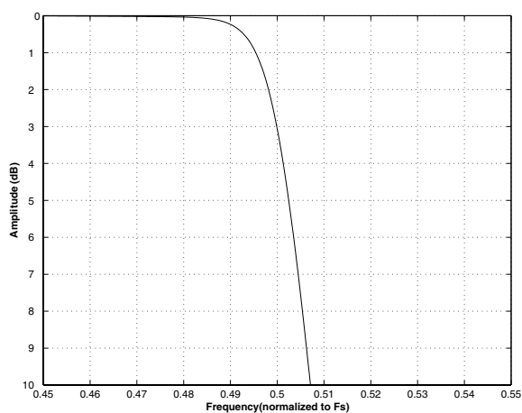
Figure 11. Single Speed (fast) Transition Band (detail)
