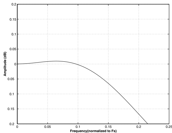
Figure 28. Quad Speed (fast) Passband Ripple
