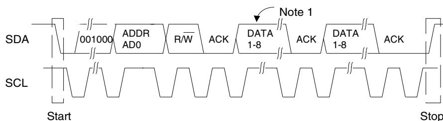
Figure 1. Control Port Timing, Two-Wire Format
