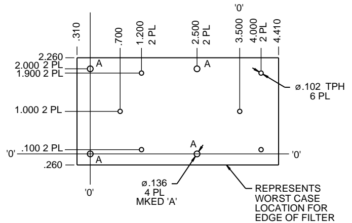
RECOMMENDED CUSTOMER MOUNTING (TOP VIEW)
