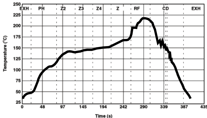
Figure 4. Solder Reflow Profile
