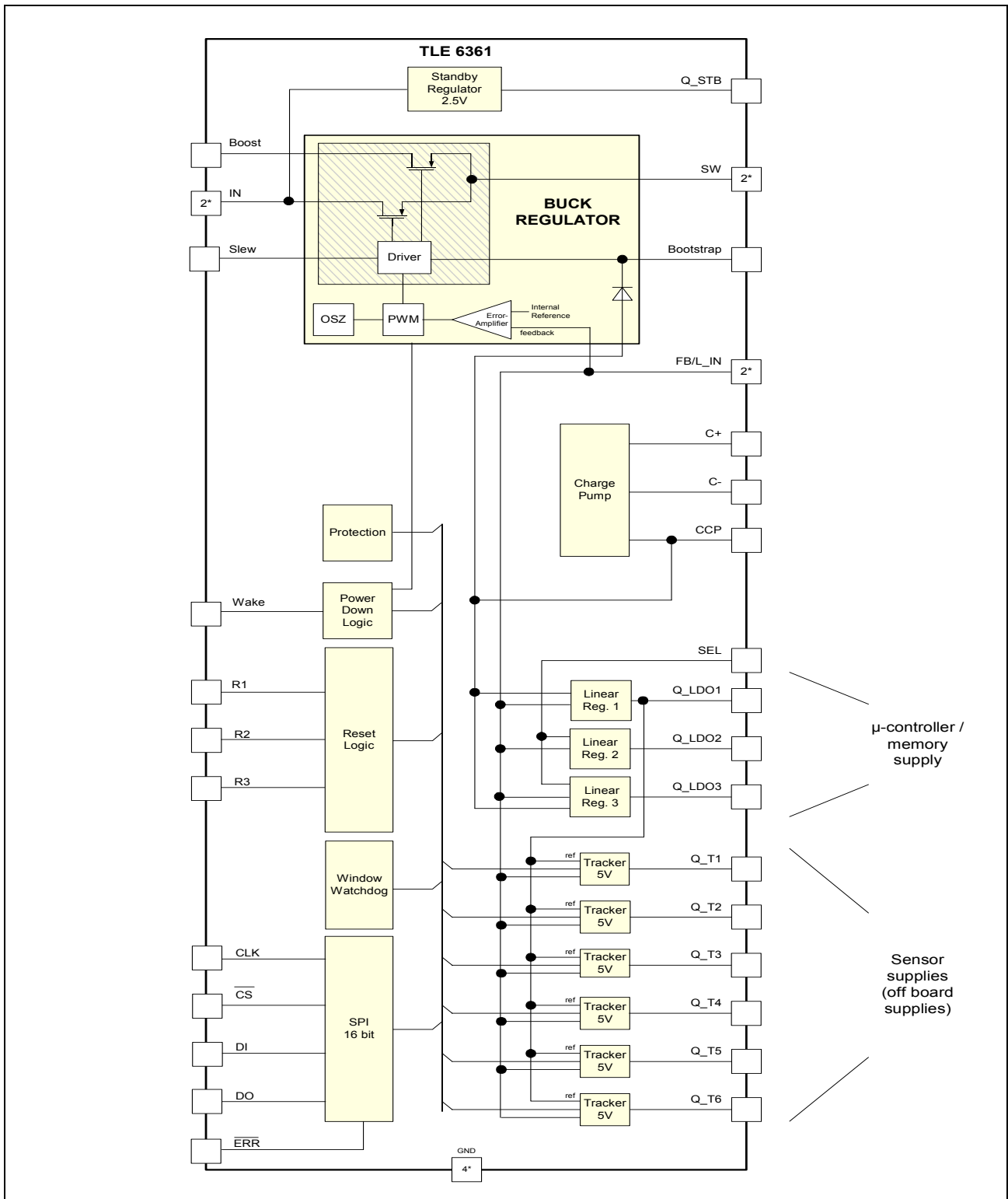
Figure 2 Block Diagram
