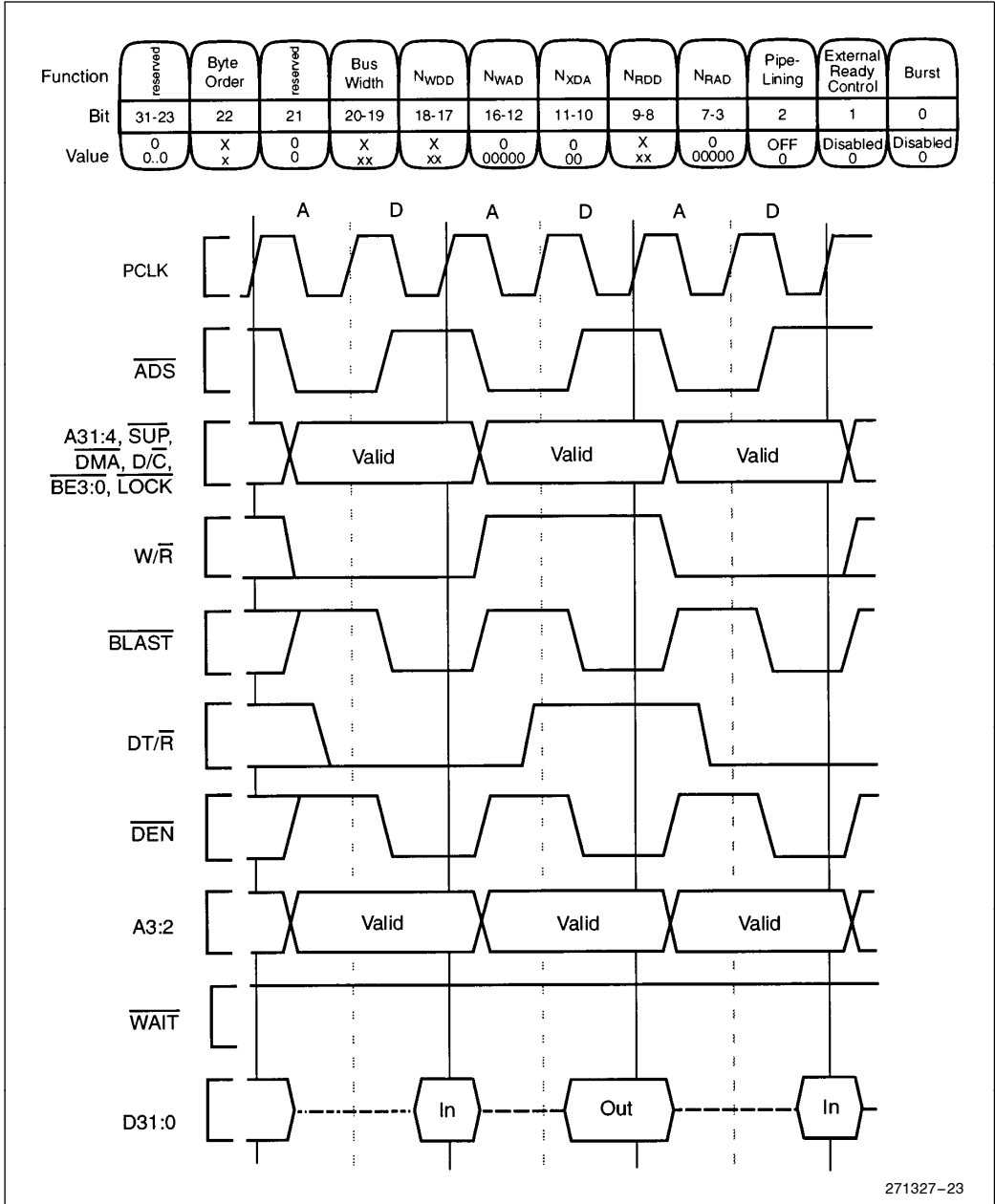
Figure 23. Non-Burst, Non-Pipelined Requests Without Wait States
