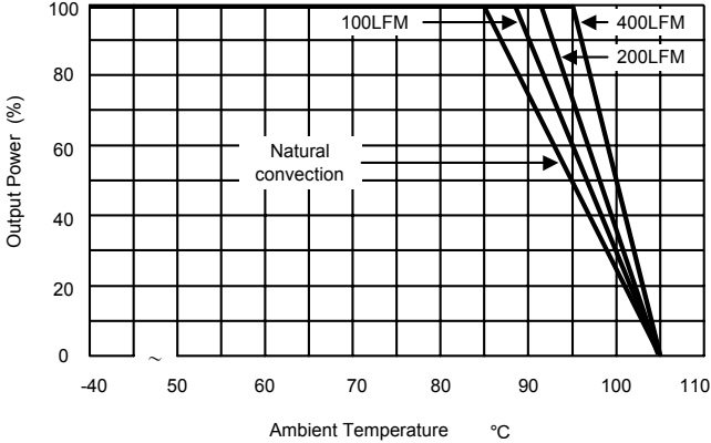
Derating Curve
