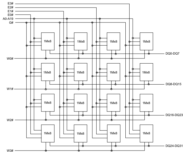
EDI7F4341MV-BNC: 4x1Mx32 80 PIN SIMM
