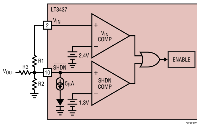
Figure 7. Undervoltage Lockout
