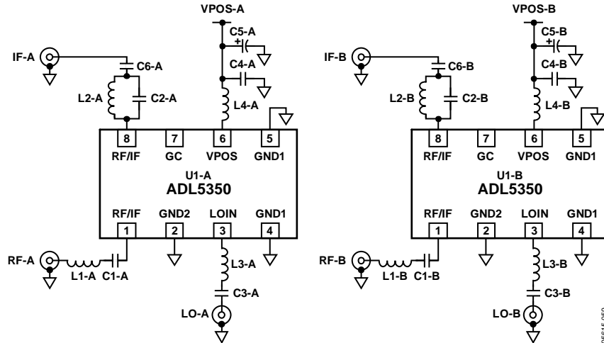
Figure 65. Evaluation Board
