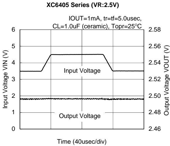
(14) Input Transient Response (Continued)
