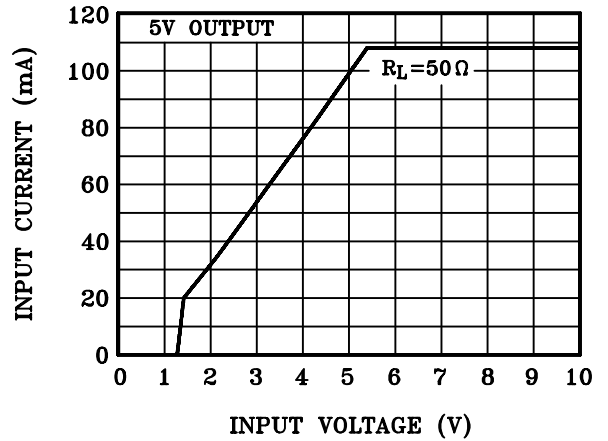
INPUT CURRENT
