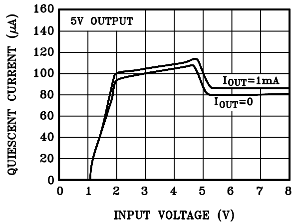
QUIESCENT CURRENT
