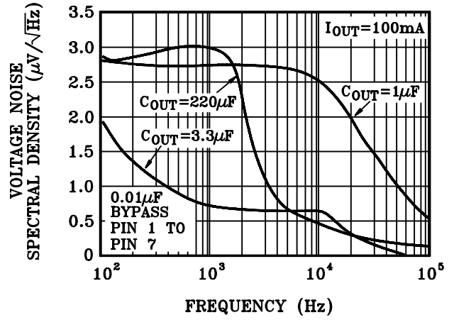
OUTPUT NOISE
