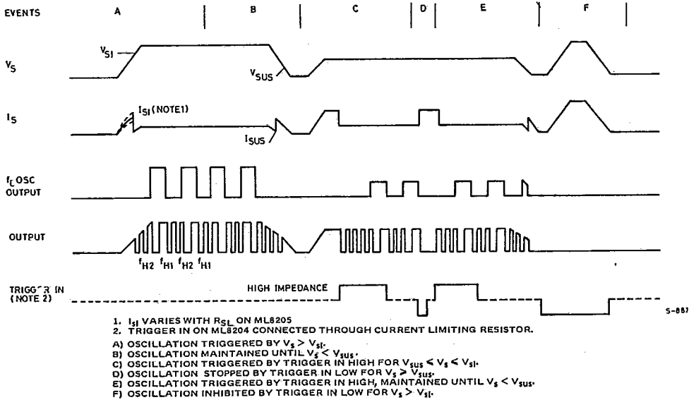
Fig. 2 - ML8204/ML8205 timing diagram
