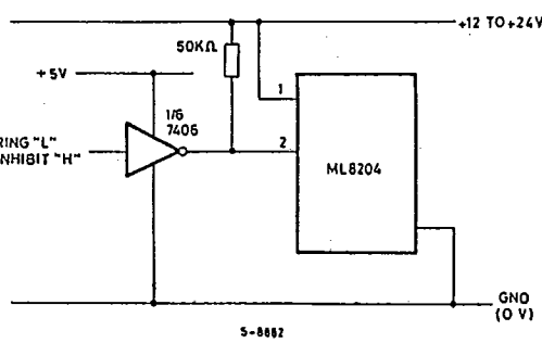
Fig. 7b - Gating the ML8204 from TTL
