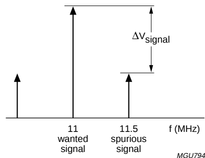
Fig.9 Base band spectrum.
