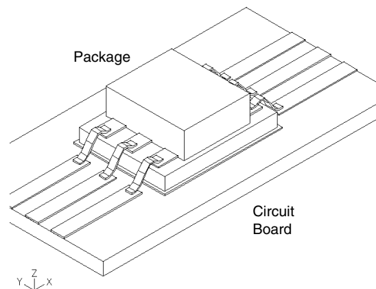
Figure 3. Surface Mount
