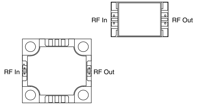
Figure 1. Co-Planar Packages
