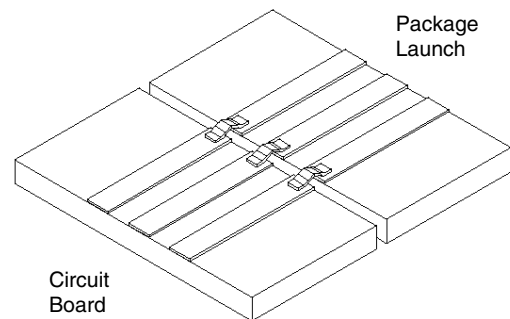
Figure 2. Microstrip Mount
