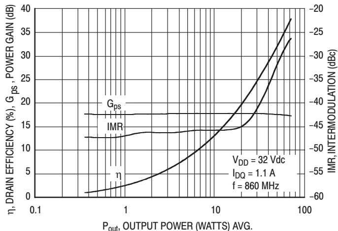
Figure 9. 8-VSB Intermodulation, Gain and Efficiency versus Output Power in Broadband Circuit
