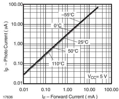
Figure 14. Photo Current vs. Forward Current
