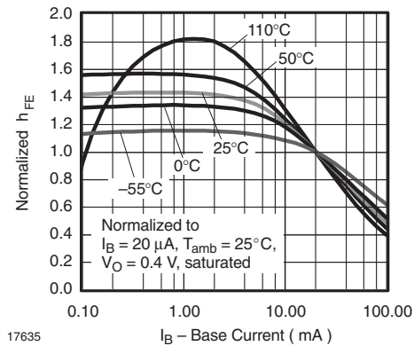
Figure 13. Normalized HFE vs. Base Current
