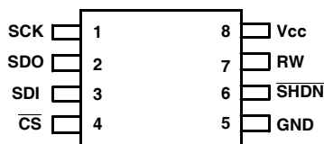
ISL22419 (8 LD MSOP) TOP VIEW
