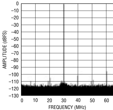
64K Point FFT, f_{IN} = 30\text{MHz} , -1dB, PGA = 0
