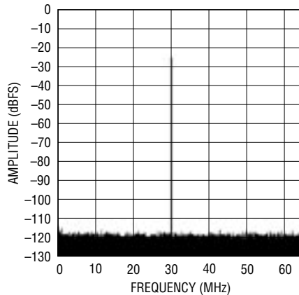
128K Point FFT, f_{IN} = 30.1\text{MHz} , -26dBFS, PGA = 0, Dither "On"
