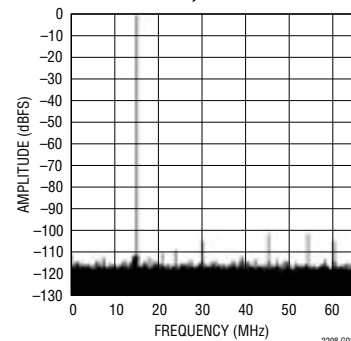
64k Point FFT, F_{IN} = 15.1\text{MHz} , -1dB, PGA = 0
