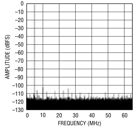
64K Point FFT, f_{IN} = 5\text{MHz} , -1dB, PGA = 0
