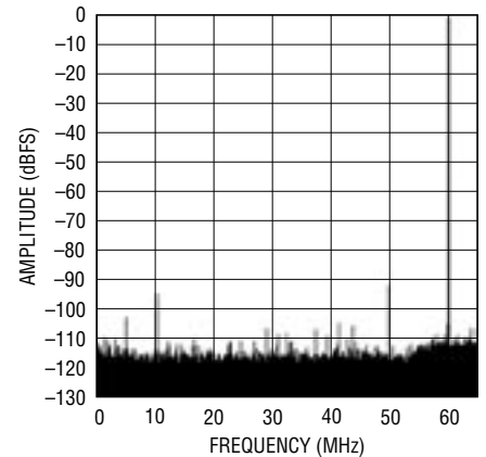
64K Point FFT, f_{IN} = 70.1\text{MHz} , -1dB, PGA = 0
