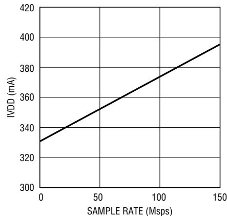
I_{VDD} vs Sample Rate, 5MHz Sine Wave, -1dB
