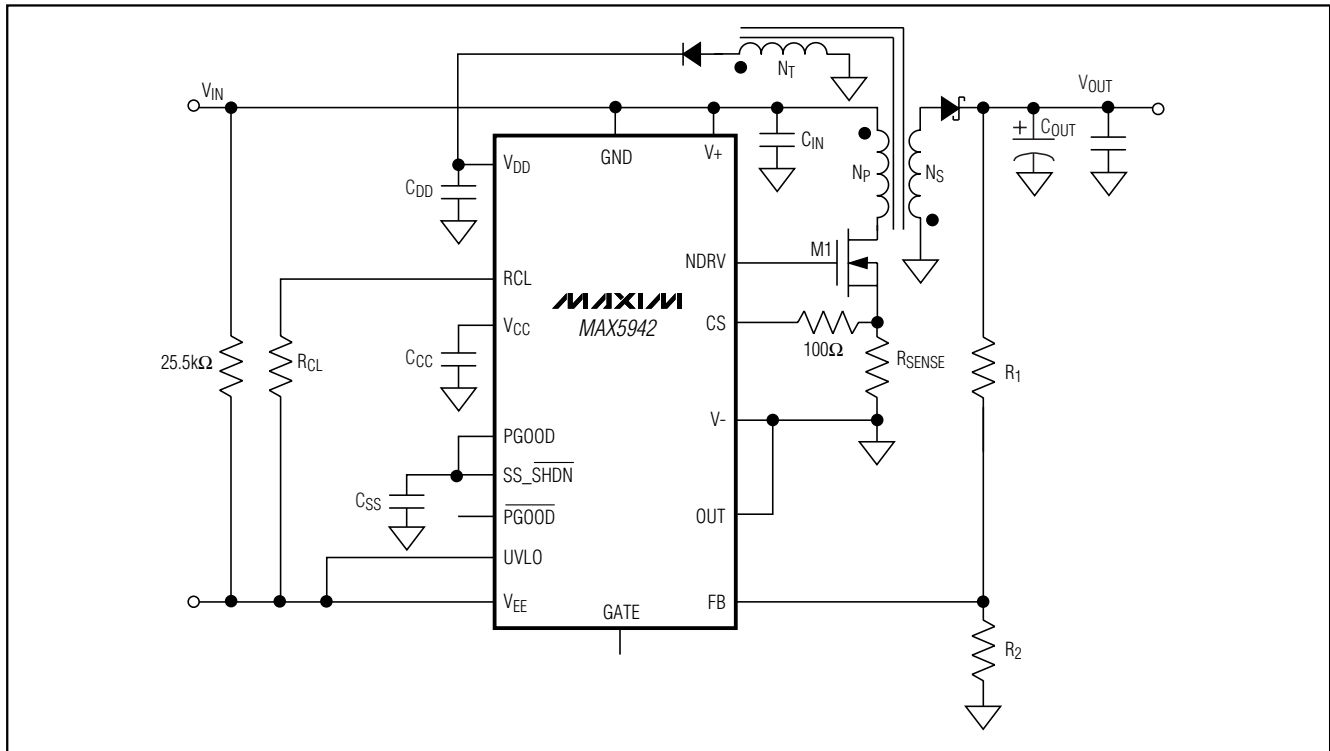
Figure 6. Flyback Converter
