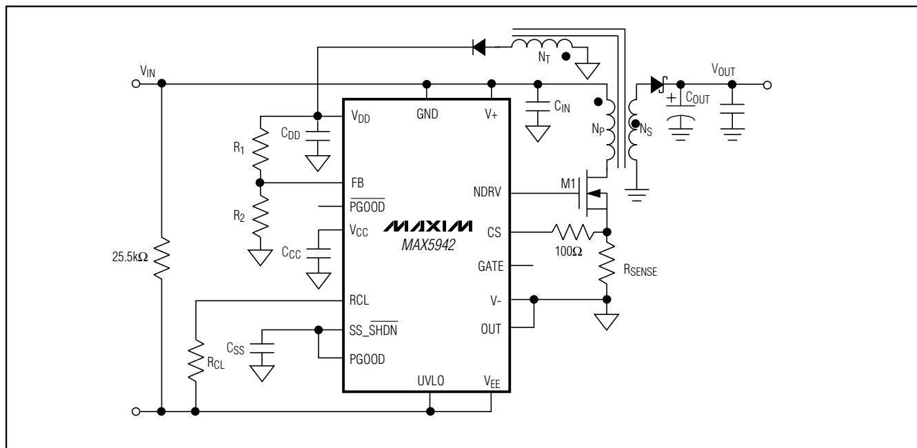
Figure 7. Flyback Converter
