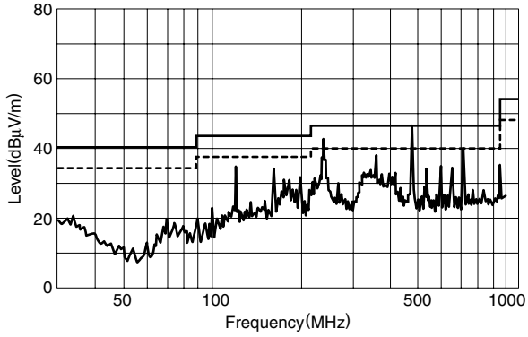
(1) Without EMC
