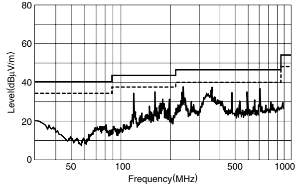
(2) With TCM1210-900-2P
