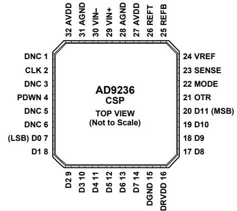
Figure 4. 32-Lead LFCSP
