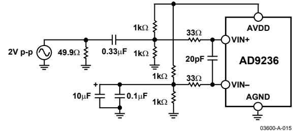
Figure 30. Single-Ended Input Configuration
