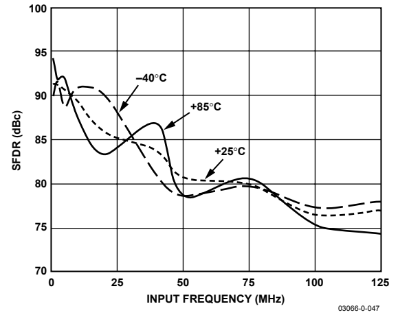
Figure 24. SFDR vs. Input Frequency
