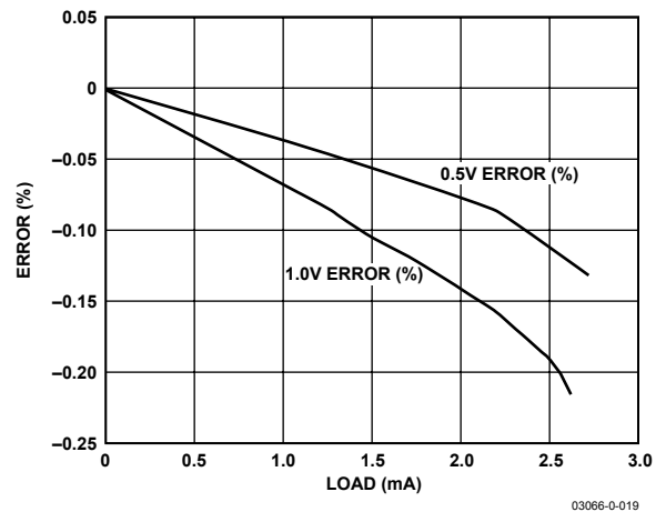
Figure 34. VREF Accuracy vs. Load
