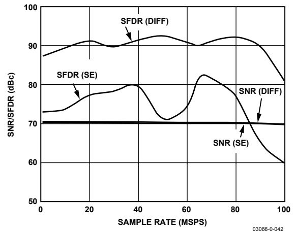
Figure 14. SNR/SFDR vs. Sample Rate @ 10 MHz
