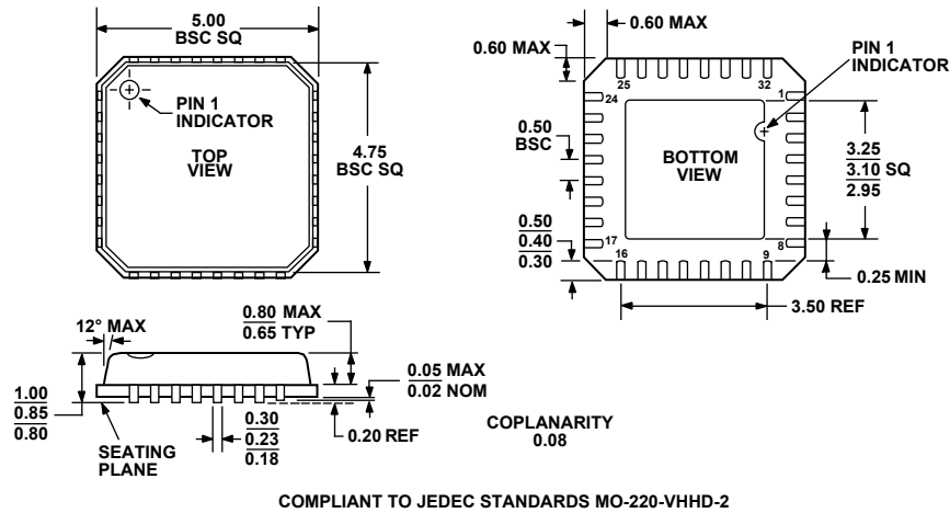
Figure 58. 32-Lead Frame Chip Scale Package [LFCSF] (CP-32-1)—Dimensions shown in millimeters
