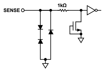
Figure 7. Equivalent SENSE Circuit
