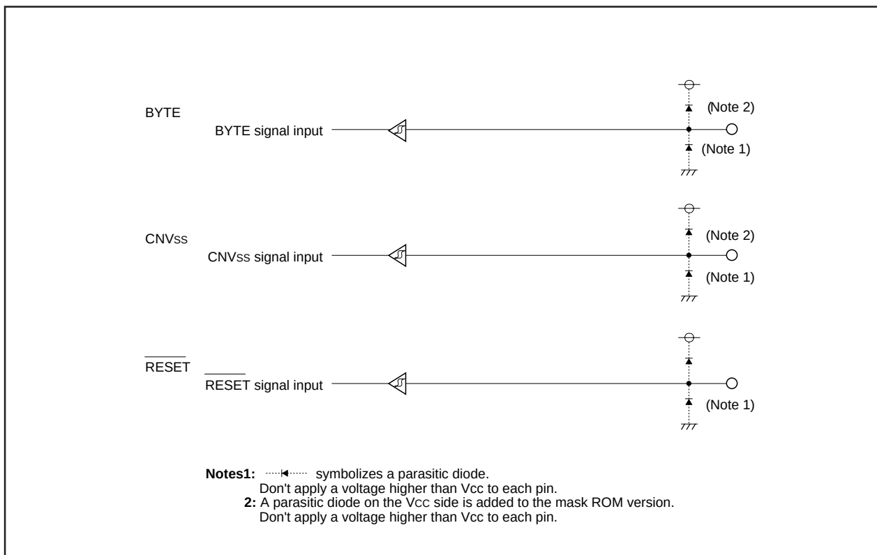
Figure 2.17.5 I/O pins
