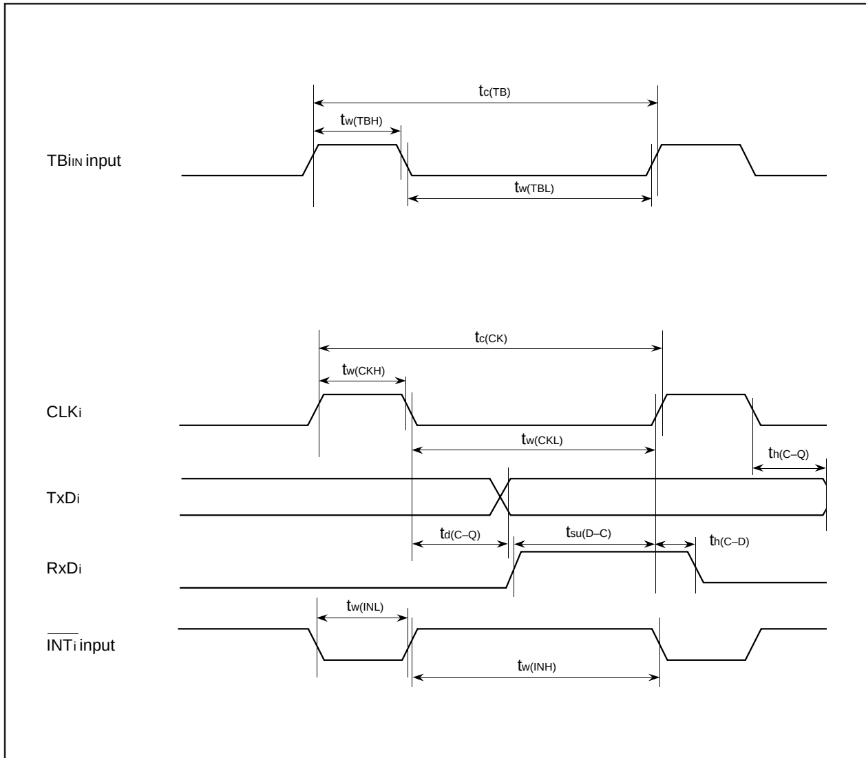
Figure 5.10.1 Timing diagram
