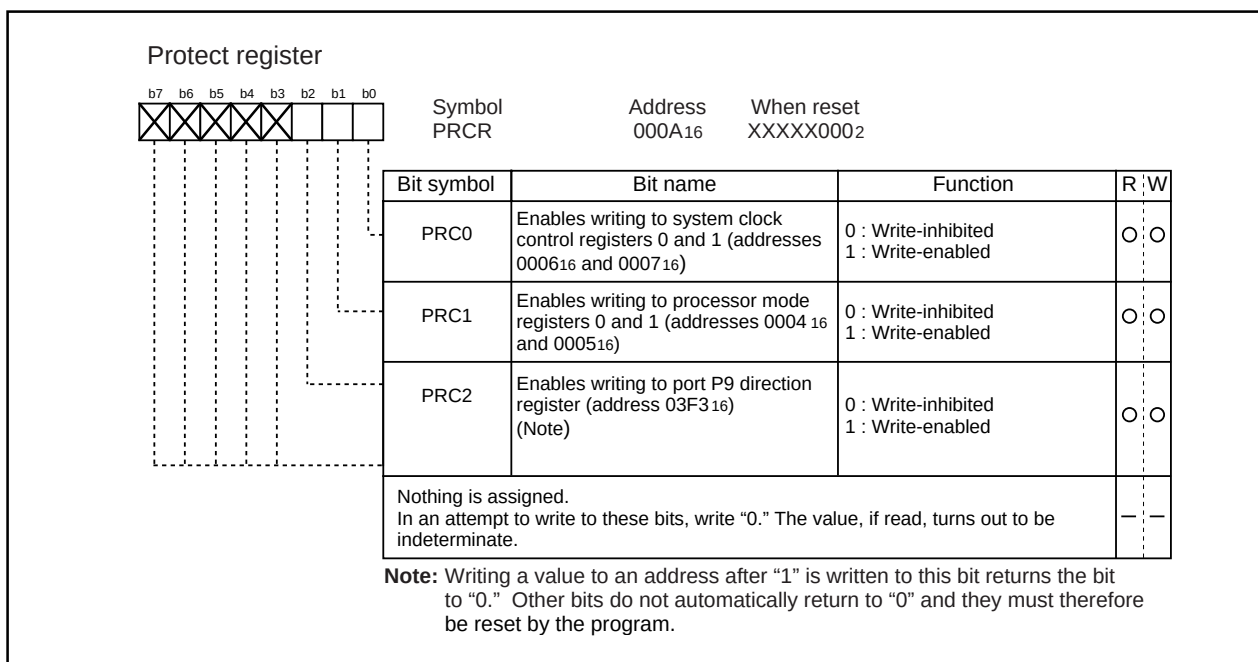
Figure 2.6.1 Protect register
