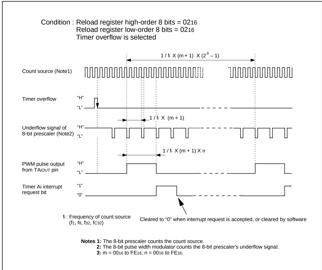
Figure 2.10.15 Example of how an 8-bit pulse width modulator operates
