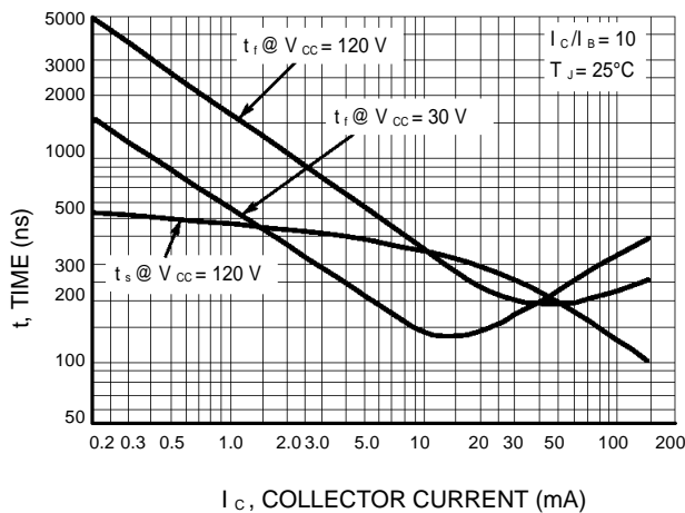
Figure 9. Turn-Off Time
