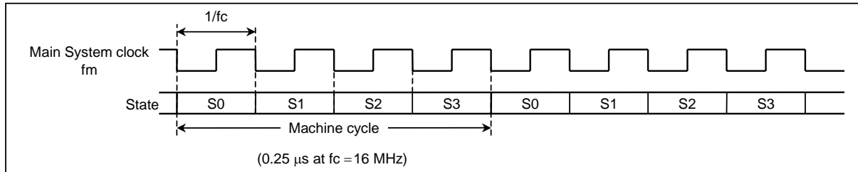
Figure 1.4.6 Machine Cycle
