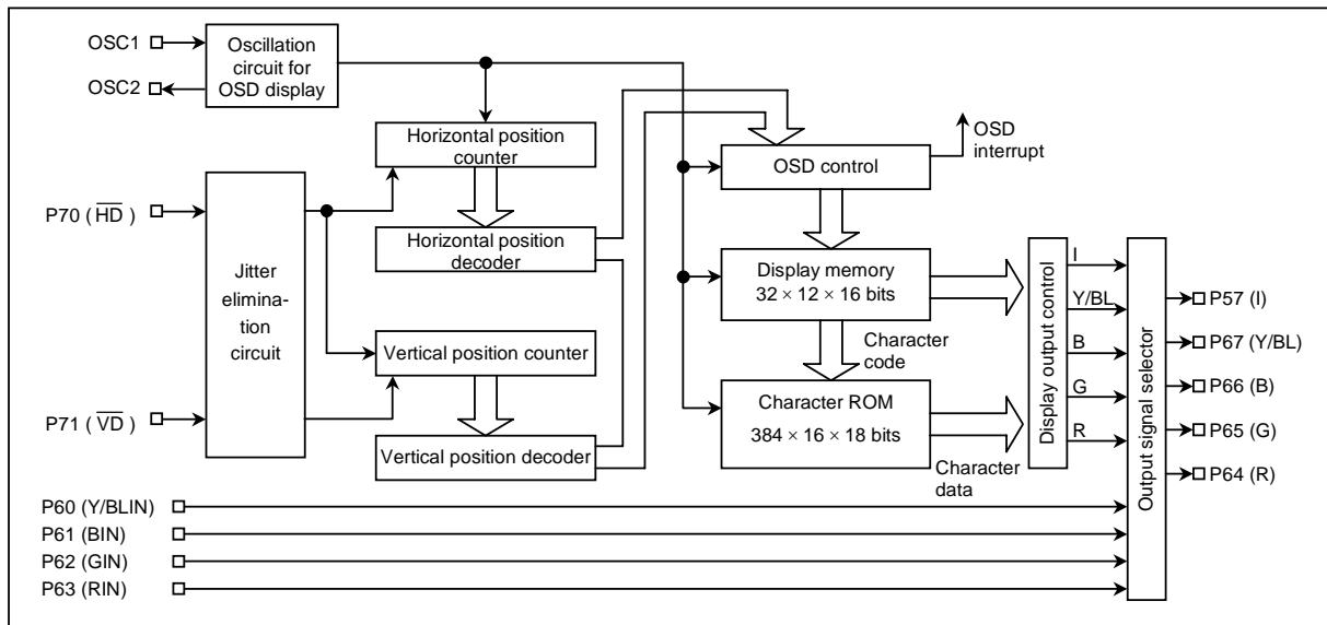
Figure 2.15.1 OSD Circuit
