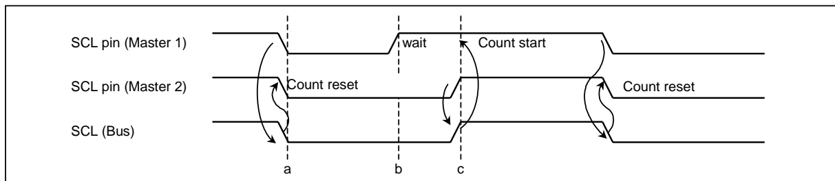
Figure 2.9.8 Clock Synchronization
