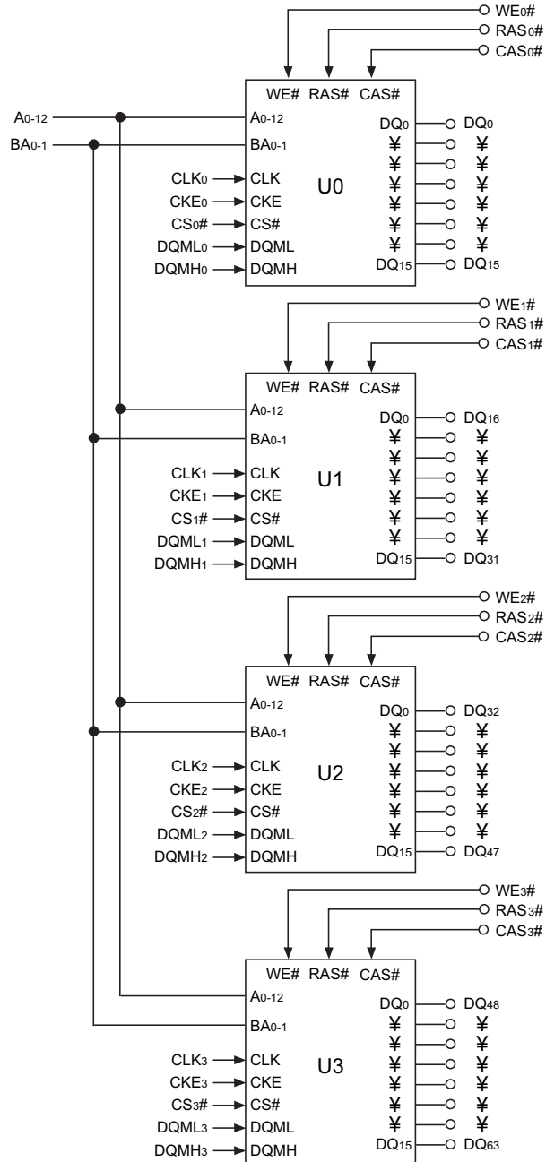
FIGURE 2 – FUNCTIONAL BLOCK DIAGRAM
