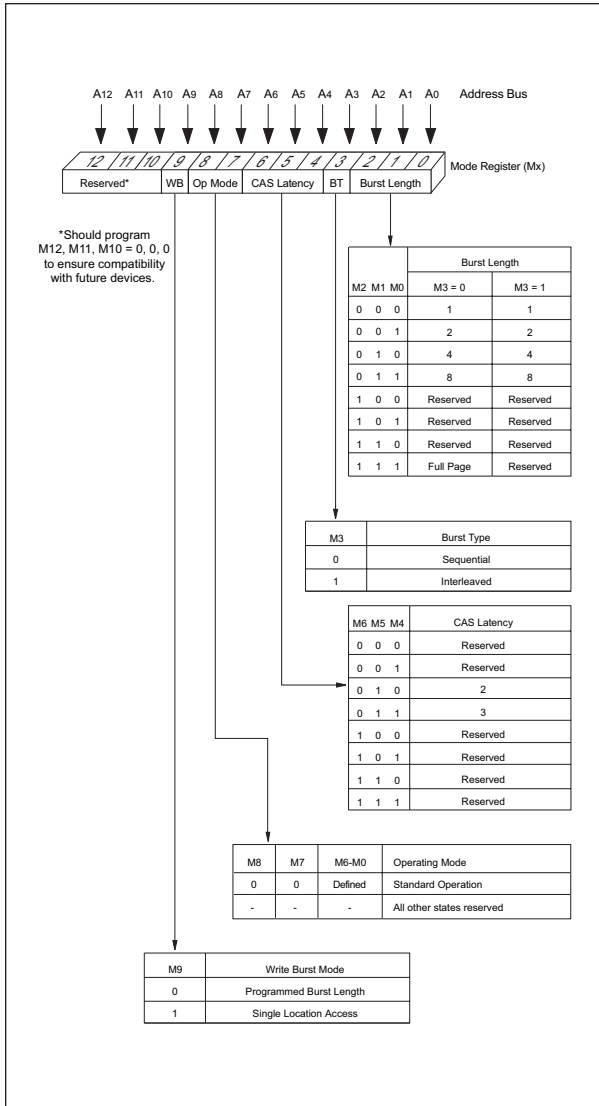
FIGURE 3 – MODE REGISTER DEFINITION
