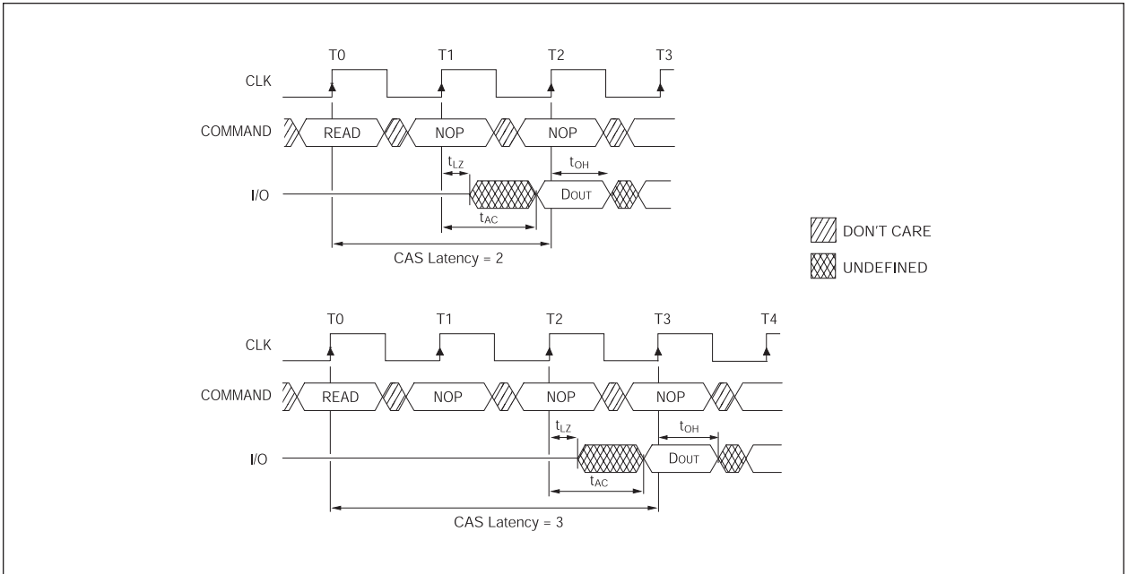
FIGURE 4 – CAS LATENCY
