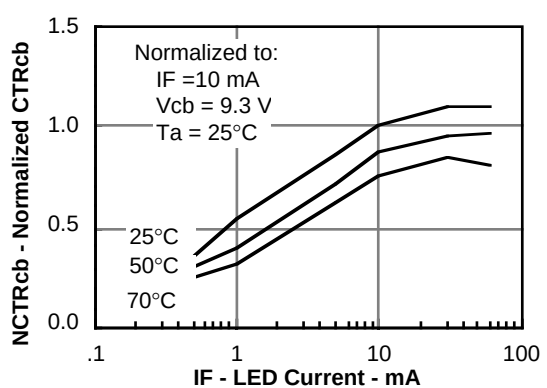
Figure 12. Normalized \text{CTR}_{cb} versus LED current and temperature
