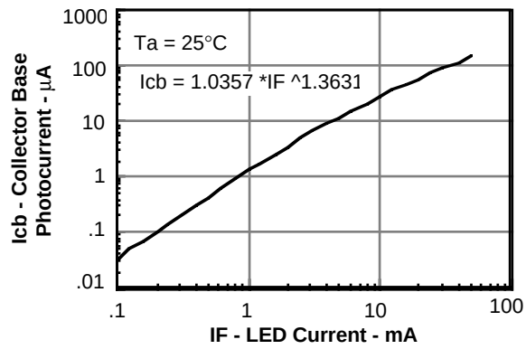
Figure 13. Collector base photocurrent versus LED current
