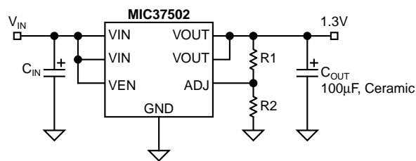
Adjustable Regulator
