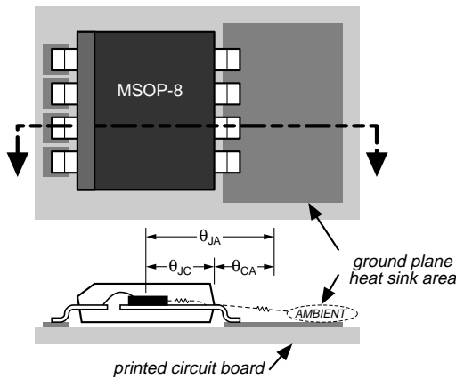
Figure 1. Thermal Resistance
