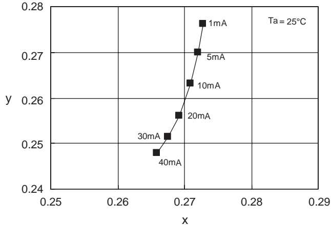
Forward Current vs. Chromaticity Coordinates
