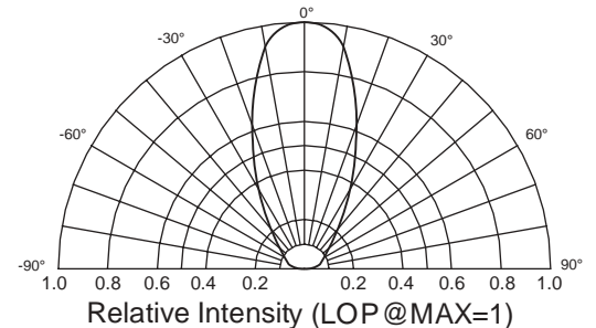
Beam Pattern
