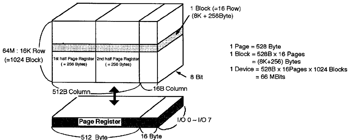
Figure 2. ARRAY ORGANIZATION
