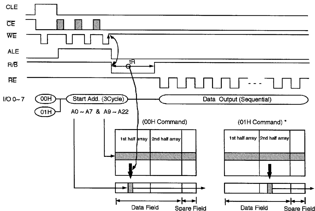
Figure 3. Read 1 Operation
