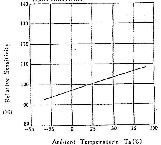
RELATIVE SENSITIVITY VS TEMPERATURE
