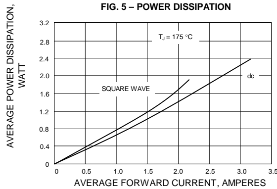
FIG. 5 - POWER DISSIPATION
