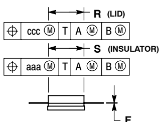
CASE 465A-06 ISSUE H NI-780S MRF6S23100HSR3
