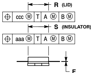
CASE 465-06 ISSUE G NI-780 MRF6S23100HR3
