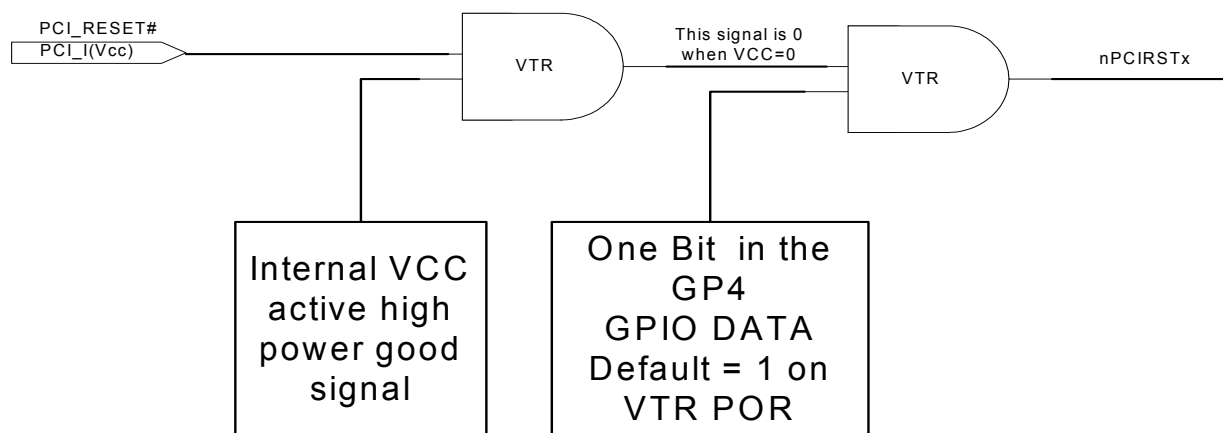
Figure 19.1 nPCIRSTx Logic
