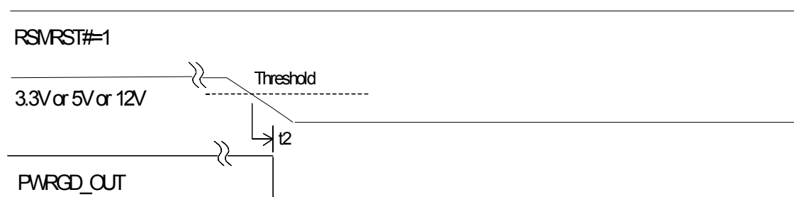
(b) Power Down Due to Drop in Power Supply
