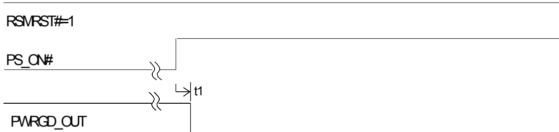
(a) Normal Power Down Due to PS_ON# Deasserted
