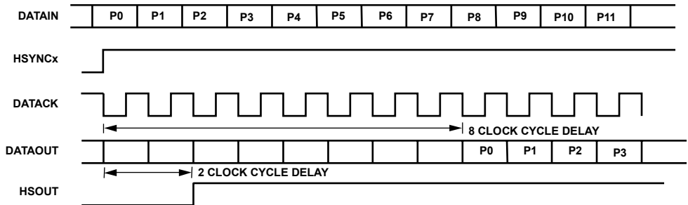
Figure 15. 4:4:4 Timing Mode
