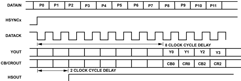
Figure 15. 4:4:4 Timing Mode
