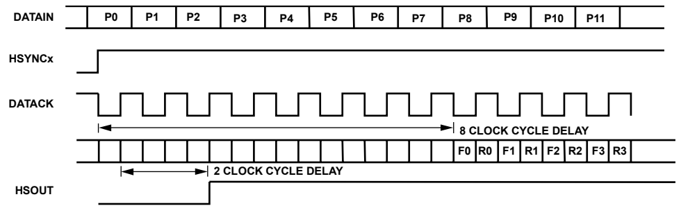
Figure 16. 4:2:2 Timing Mode
