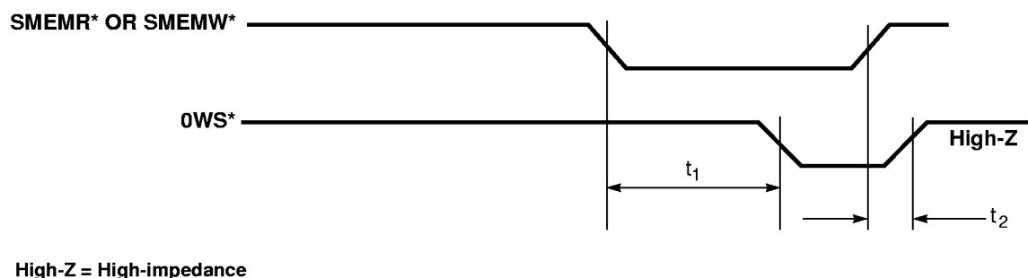
Figure 7-9. OWS* Timing (ISA Bus — CL-GD5434 only)
