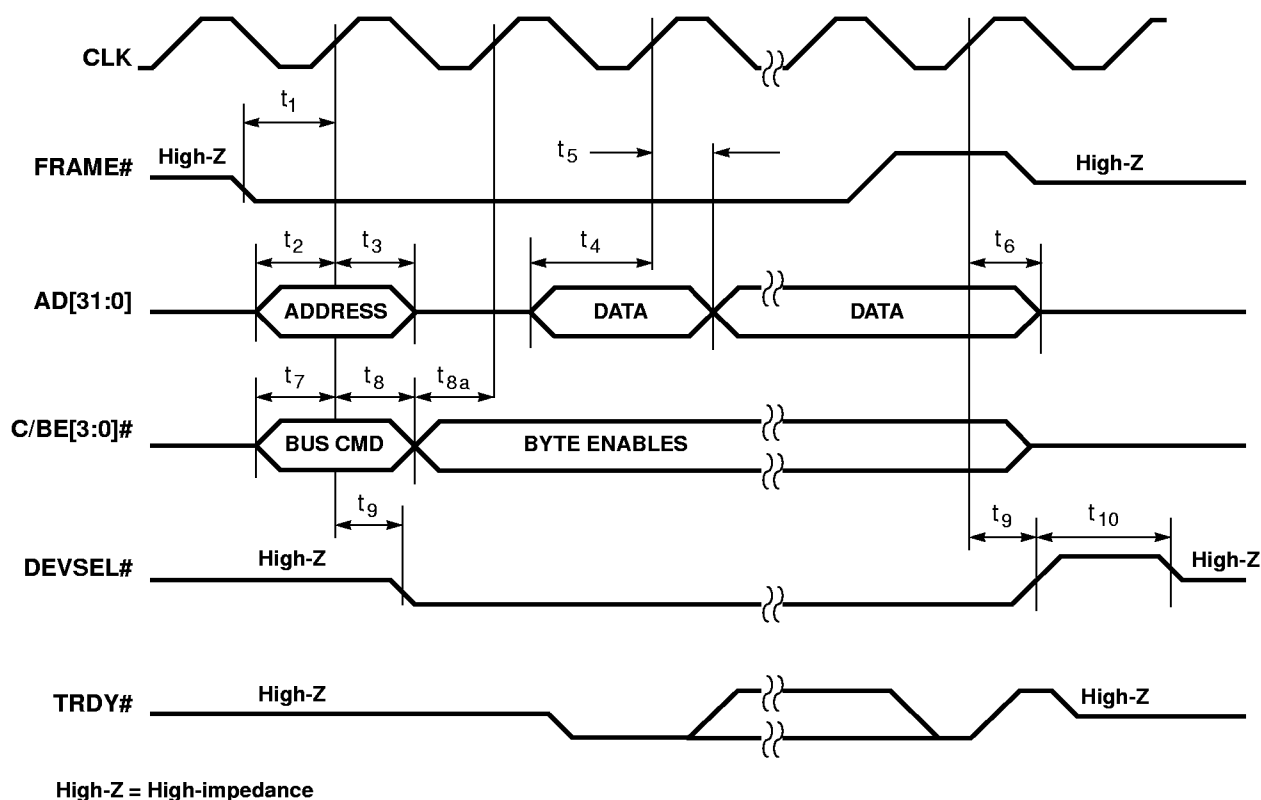
Figure 7-17. FRAME#, DEVSEL#, AD[31:0], and C/BE[3:0]# (PCI Bus)
