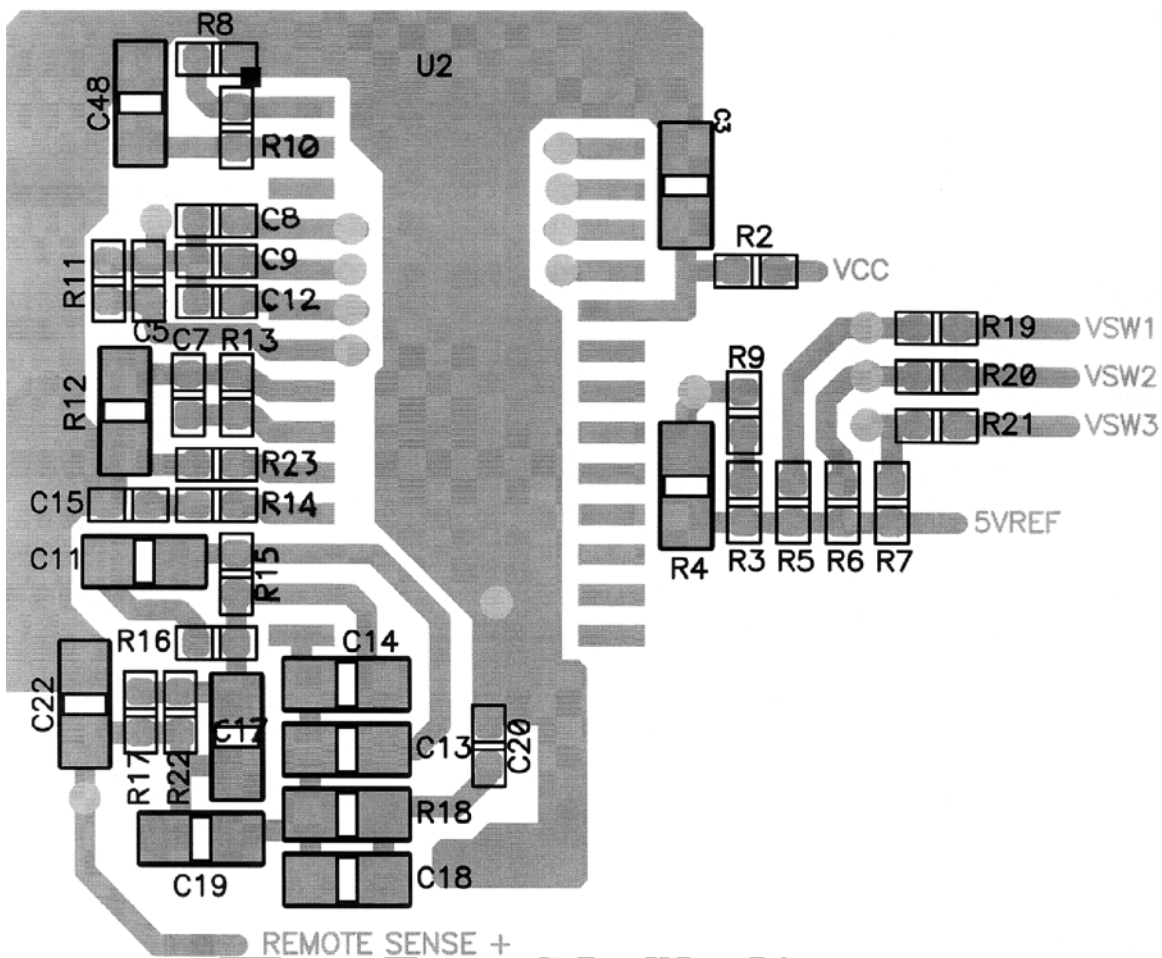
Figure 50. Sample Layout
