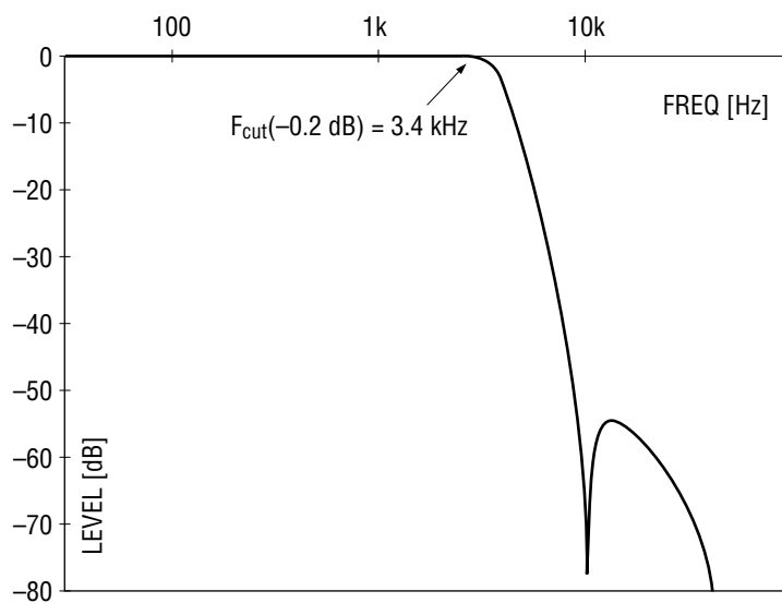
Figure 5 MSM7557 Splatter Filter
