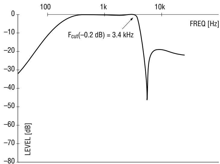
Figure 6 MSM7557 RBPF
