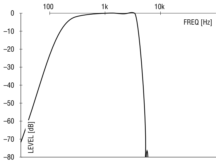
Figure 10 MSM7557 Transmit and Receive Total
