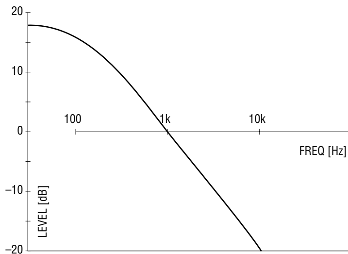
Figure 7 MSM7557 De-Emphasis
