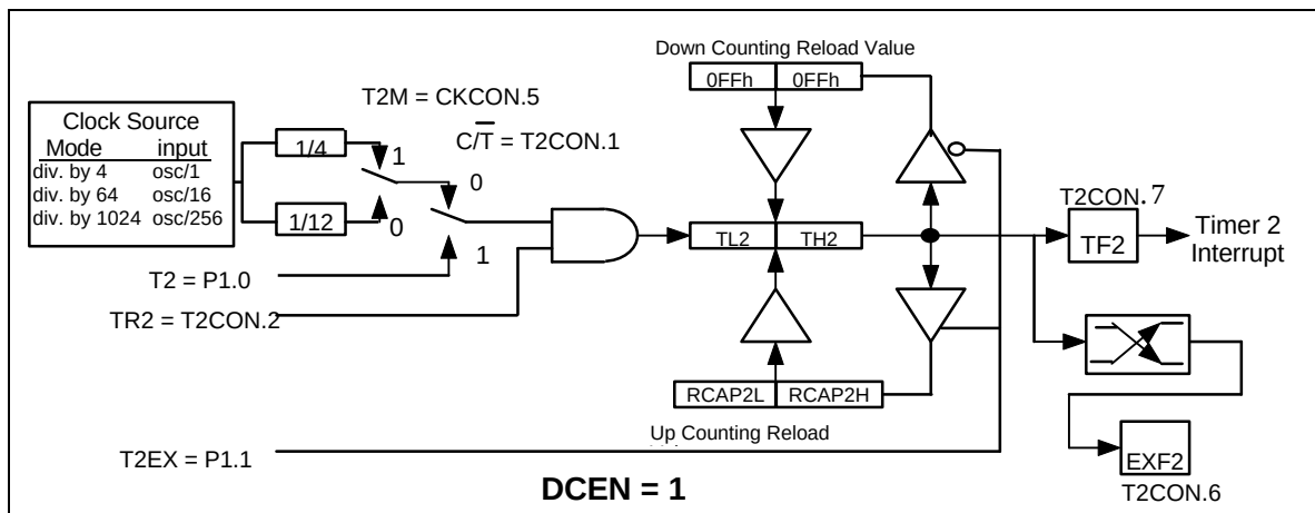
Figure 16. 16-Bit Auto-reload Up/Down Counter
