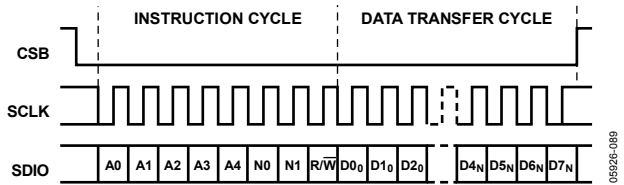
Figure 75. Serial Register Interface Timing, LSB First Write
