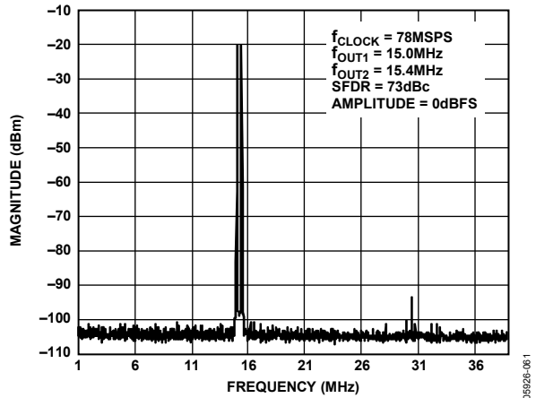
Figure 55. AD9705 Dual-Tone SFDR
