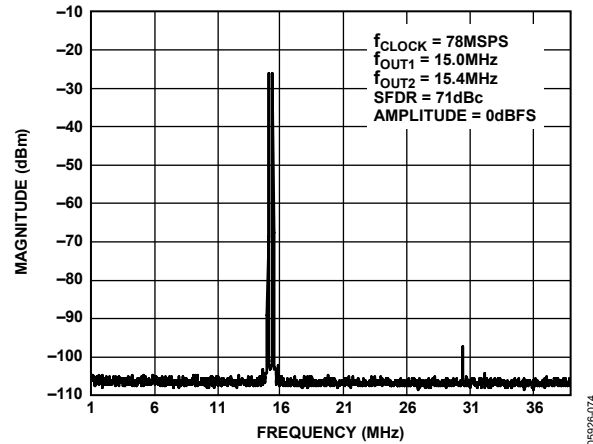
Figure 68. AD9705 Dual-Tone SFDR
