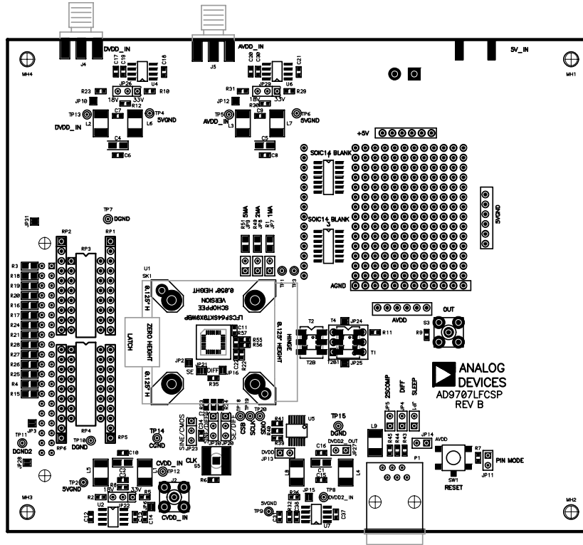
Figure 98. Assembly—Primary Side
