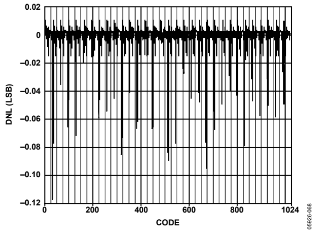
Figure 62. AD9705 Typical Uncalibrated DNL
