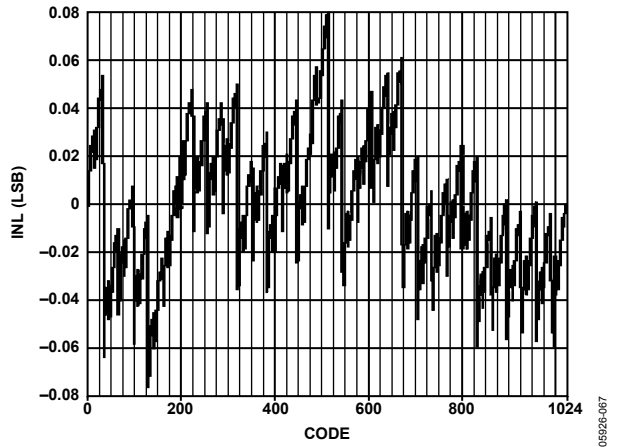
Figure 61. AD9705 Typical Uncalibrated INL
