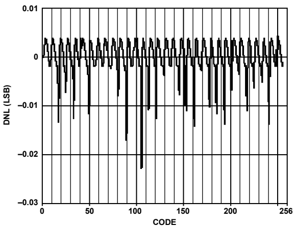
Figure 60. AD9704 Typical Uncalibrated DNL
