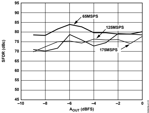
Figure 14. Single-Tone SFDR vs. A_{OUT} @ f_{OUT} = f_{CLOCK}/5
