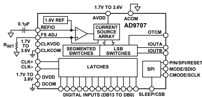
Figure 72. Simplified Block Diagram
