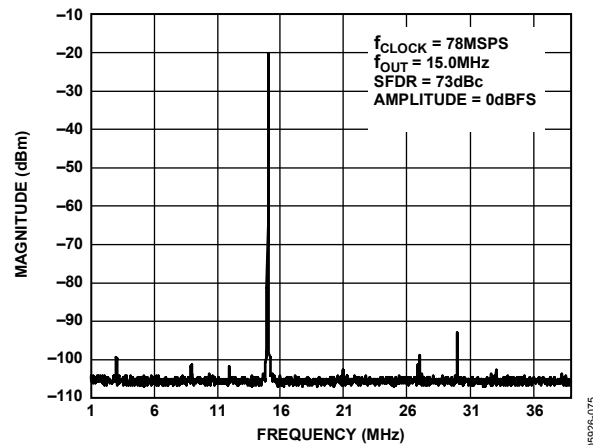
Figure 69. AD9706 Single-Tone SFDR
