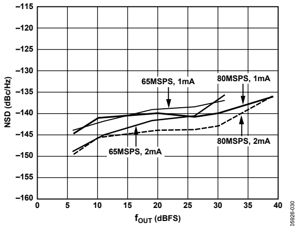
Figure 34. NSD vs. f_{OUT} , f_{CLOCK} , and I_{OUTS} @ 0 \text{ dBFS}
