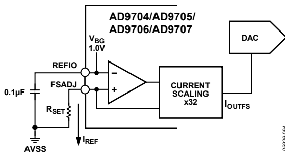
Figure 79. Internal Reference Configuration
