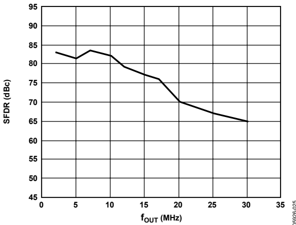
Figure 29. SFDR vs. f_{OUT} @ 65 MSPS
