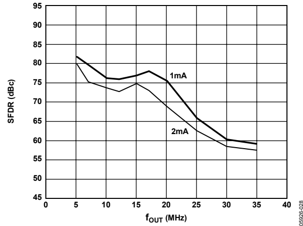
Figure 32. SFDR vs. f_{OUT} and I_{OUTFS} @ 80 MSPS
