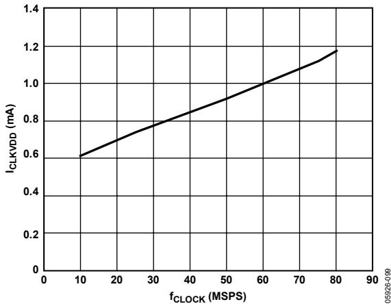
Figure 87. I CLKVDD vs. f CLOCK (Differential Clock Mode) @ CLKVDD = 1.8 V
