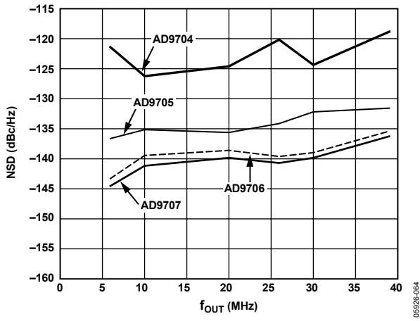
Figure 58. AD9704, AD9705, AD9706 NSD vs. f_{OUT} @ 0 dBFS
