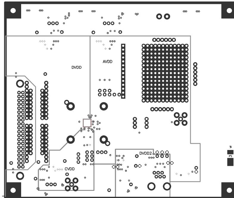
Figure 103. Layer 3—Power Plane
