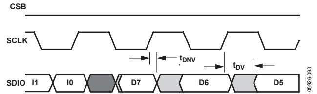
Figure 78. Timing Diagram for SPI Register Read
