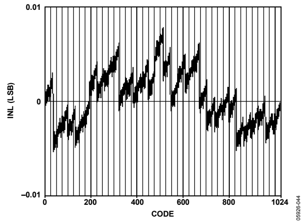
Figure 48. AD9705 Typical Uncalibrated INL
