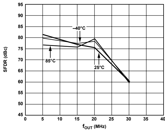
Figure 41. SFDR vs. Temperature @ 80 MSPS
