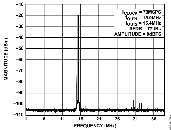
Figure 43. Dual-Tone SFDR
