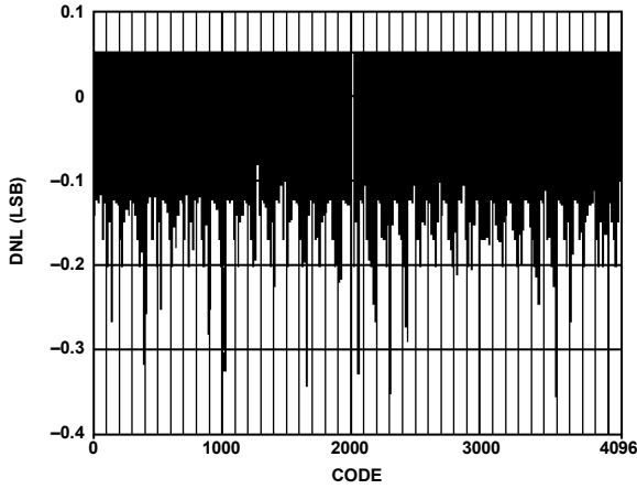
Figure 64. AD9706 Typical Uncalibrated DNL
