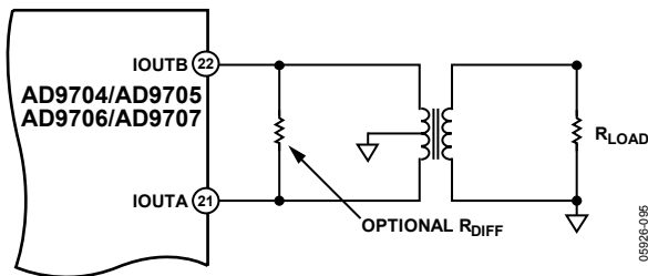
Figure 90. Differential Output Using a Transformer
