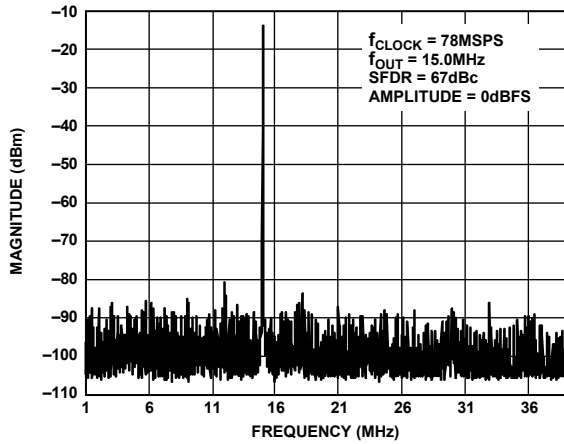
Figure 52. AD9704 Single-Tone SFDR
