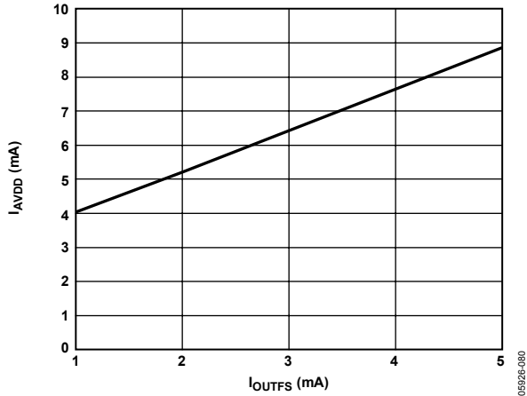
Figure 82. I_{AVDD} vs. I_{OUTFS} @ AVDD = 3.3\text{ V}
