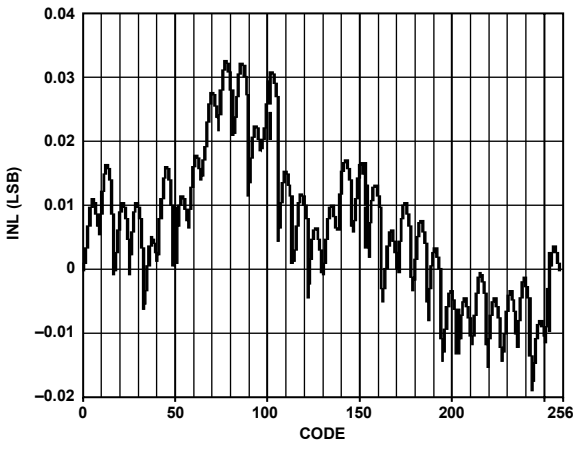
Figure 59. AD9704 Typical Uncalibrated INL
