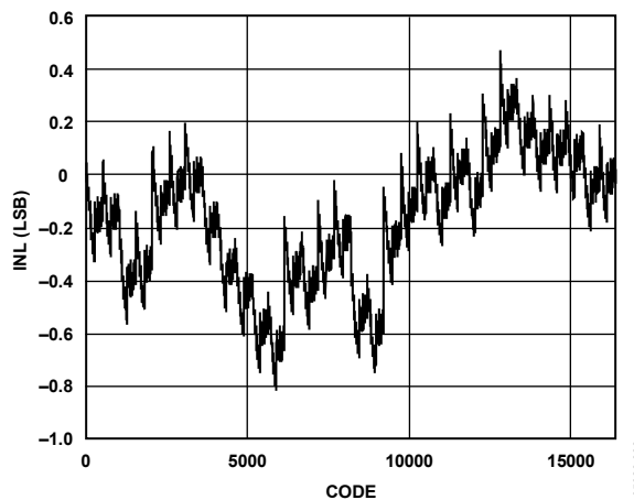
Figure 21. Typical Calibrated INL
