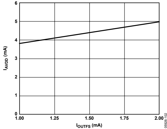
Figure 83. I_{AVDD} vs. I_{OUTFS} @ AVDD = 1.8\text{ V}
