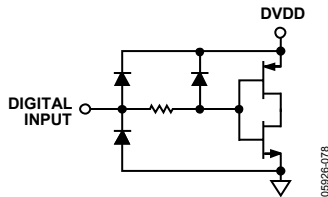
Figure 80. Equivalent Digital Input
