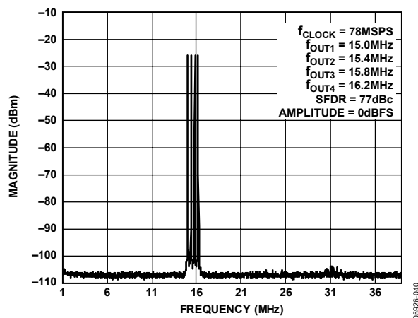
Figure 44. Four-Tone SFDR
