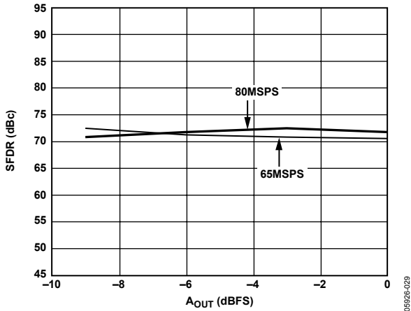
Figure 33. Single-Tone SFDR vs. A_{OUT} @ f_{OUT} = f_{CLOCK}/5
