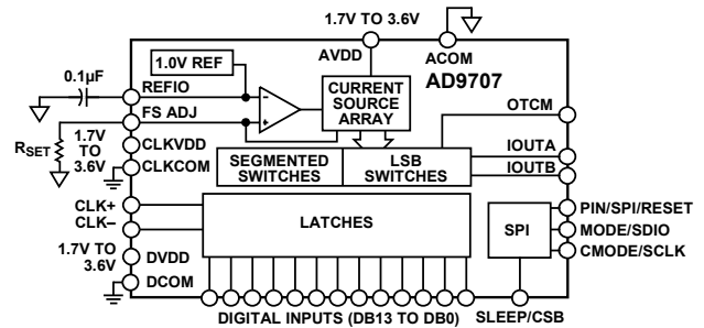
Figure 1. AD9707
