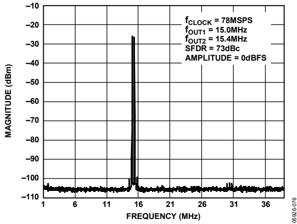
Figure 70. AD9706 Dual-Tone SFDR
