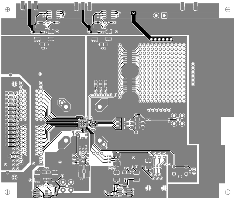
Figure 100. Layer 1—Primary Side
