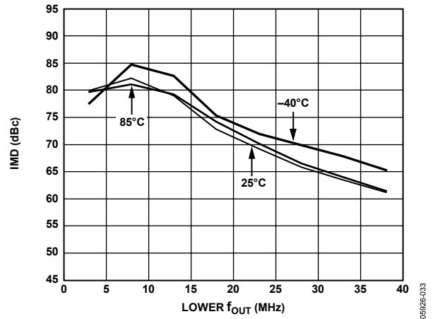
Figure 37. Dual-Tone IMD vs. f_{OUT} and Temperature @ 80 \text{ MSPS} , I_{OUTS} = 1 \text{ mA} and 0 \text{ dBFS}
