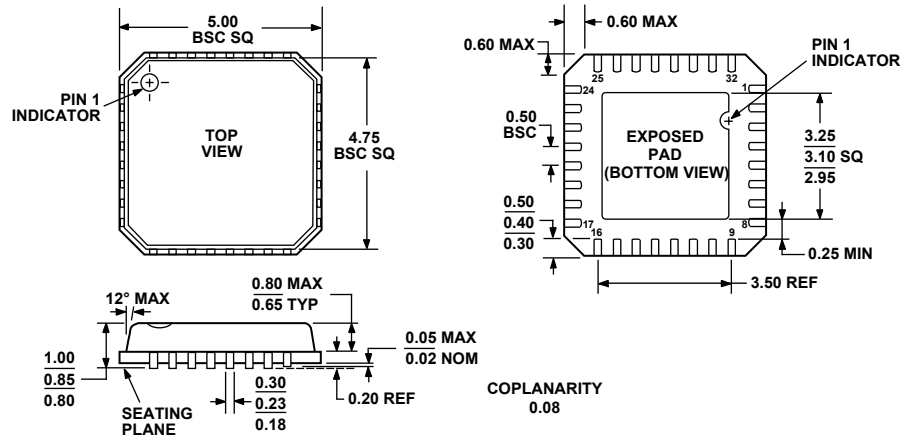
Figure 104. 32-Lead Lead Frame Chip Scale Package [LFCSP_VQ] 5 mm × 5 mm, Very Thin Quad (CP-32-2)
