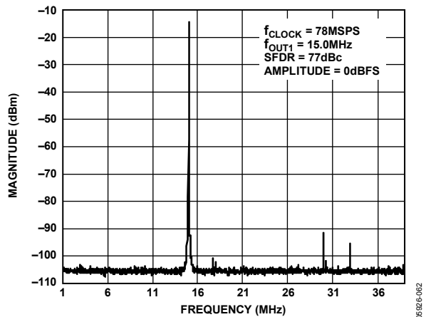
Figure 56. AD9706 Single-Tone SFDR
