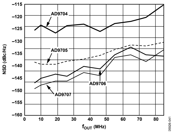
Figure 45. AD9704, AD9705, AD9706 NSD vs. f_{OUT} @ 0 dBFS
