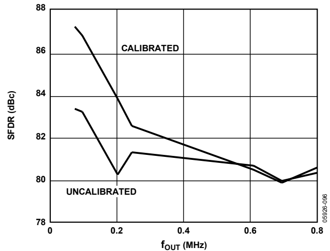
Figure 88. AD9707 SFDR vs. f OUT @ 175 MSPS and I OUTFS = 2 mA
