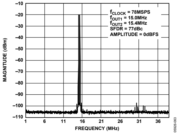
Figure 57. AD9706 Dual-Tone SFDR
