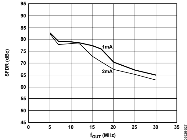
Figure 31. SFDR vs. f_{OUT} and I_{OUTFS} @ 65 MSPS
