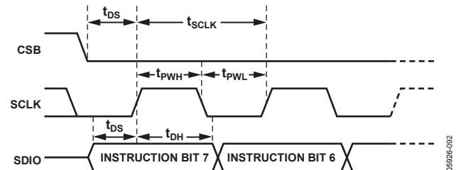
Figure 77. Timing Diagram for SPI Register Write
