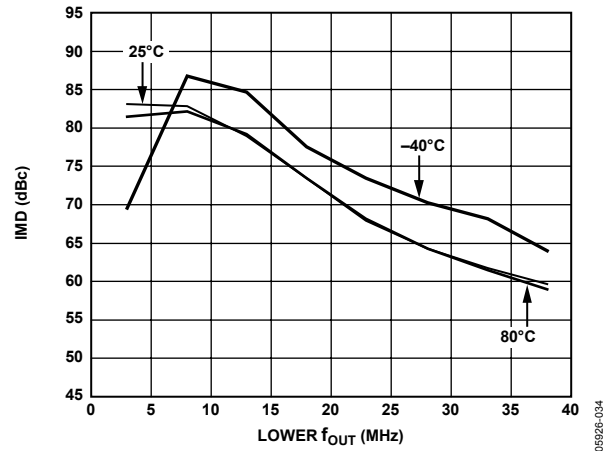
Figure 38. Dual-Tone IMD vs. f_{OUT} and Temperature @ 80 \text{ MSPS} , I_{OUTS} = 2 \text{ mA} and 0 \text{ dBFS}
