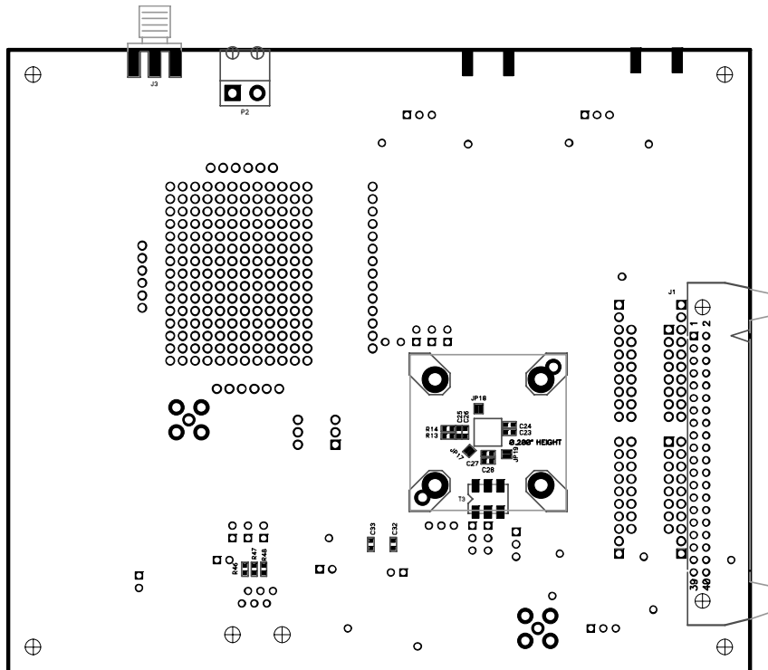
Figure 99. Assembly—Secondary Side
