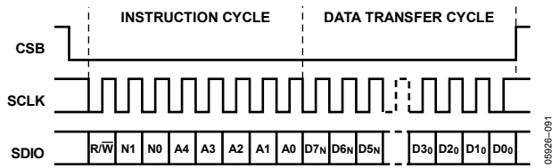
Figure 73. Serial Register Interface Timing, MSB First Write
