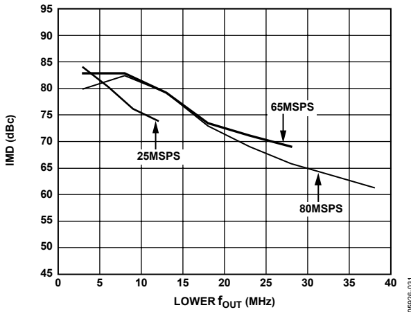
Figure 35. Dual-Tone IMD vs. f_{OUT} @ I_{OUTS} = 1 \text{ mA} and 0 \text{ dBFS}
