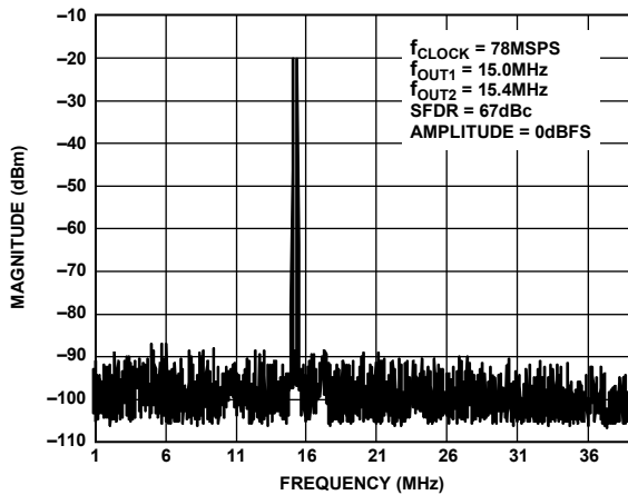
Figure 53. AD9704 Dual-Tone SFDR
