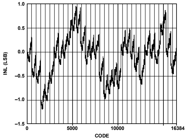
Figure 39. Typical Uncalibrated INL
