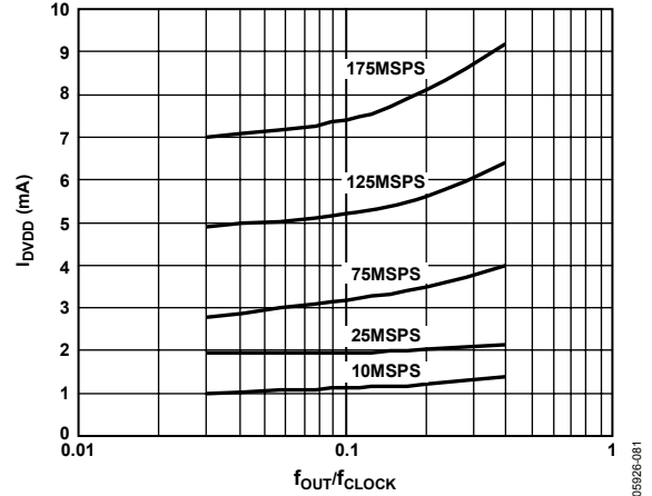
Figure 84. I_{DVDD} vs. f_{OUT}/f_{CLOCK} Ratio @ DVDD = 3.3\text{ V}
