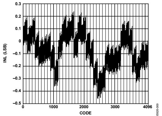
Figure 63. AD9706 Typical Uncalibrated INL
