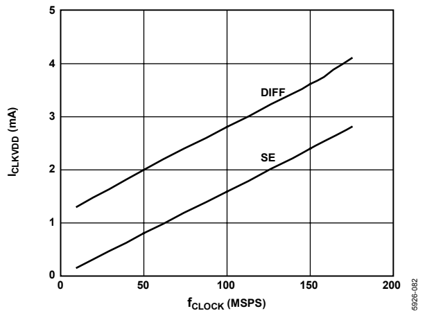
Figure 86. I_{CLKVDD} vs. f_{CLOCK} @ CLKVDD = 3.3\text{ V}
