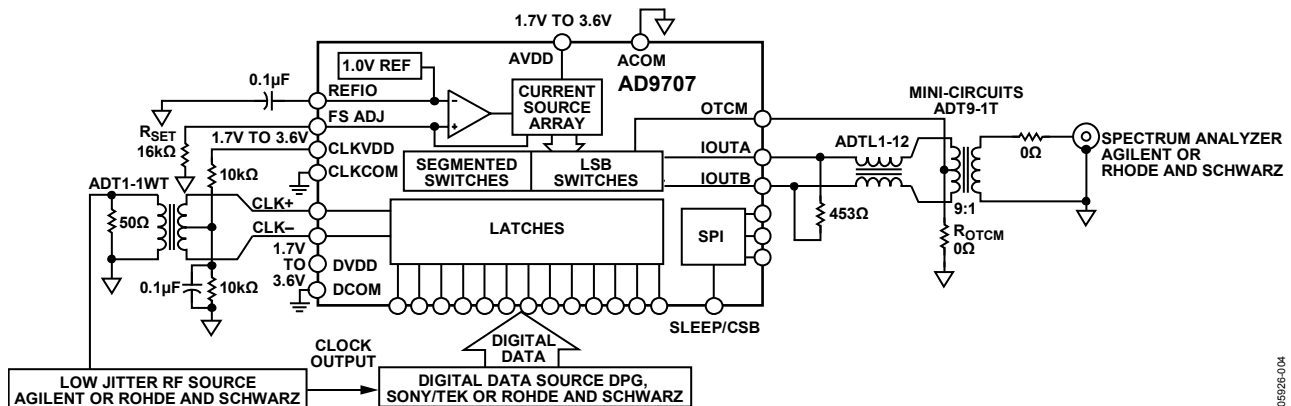
Figure 71. Basic AC Characterization Test Setup
