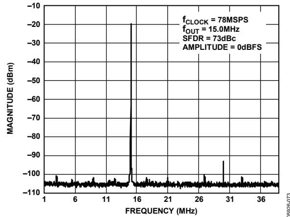
Figure 67. AD9705 Single-Tone SFDR
