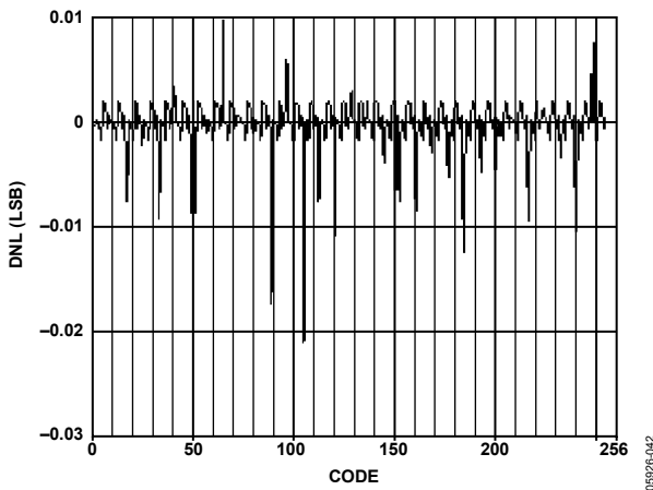
Figure 47. AD9704 Typical Uncalibrated DNL
