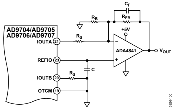
Figure 91. Single-Supply Single-Ended Buffer
