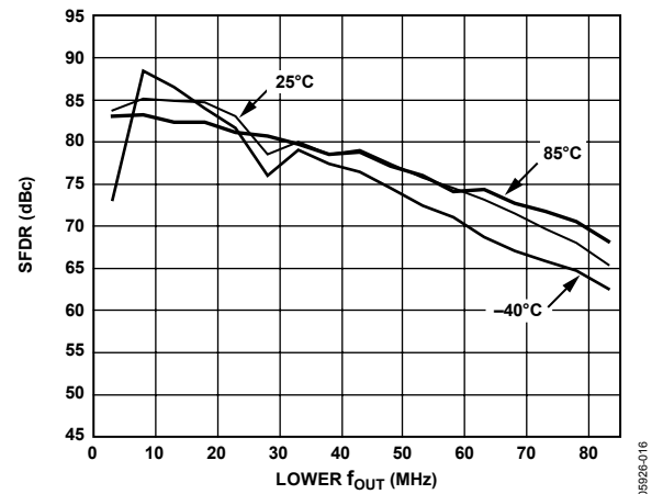
Figure 18. Dual-Tone IMD vs. f_{OUT} and Temperature @ 0 dBFS
