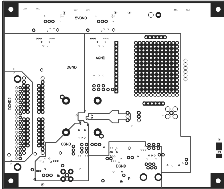
Figure 102. Layer 2—Ground Plane
