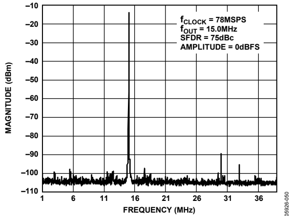
Figure 54. AD9705 Single-Tone SFDR
