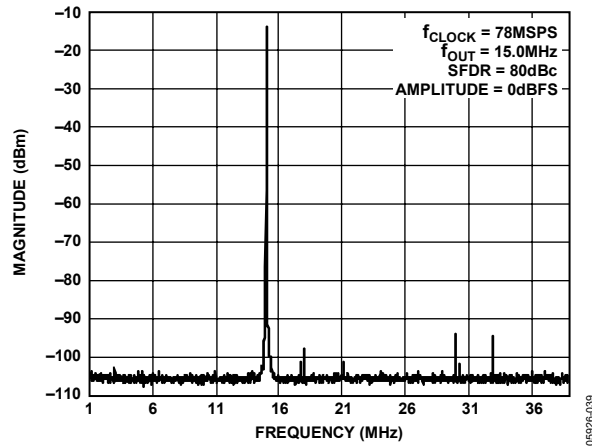
Figure 42. Single-Tone SFDR
