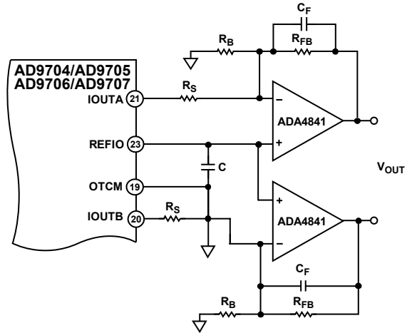
Figure 92. Single-Supply Differential Buffer
