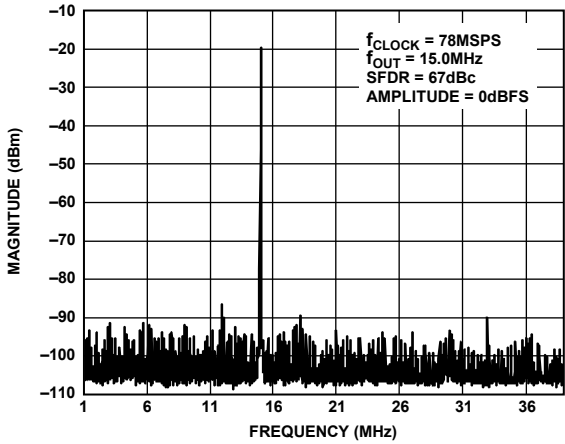
Figure 65. AD9704 Single-Tone SFDR
