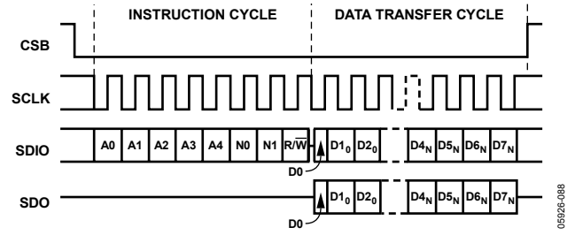
Figure 76. Serial Register Interface Timing, LSB First Read
