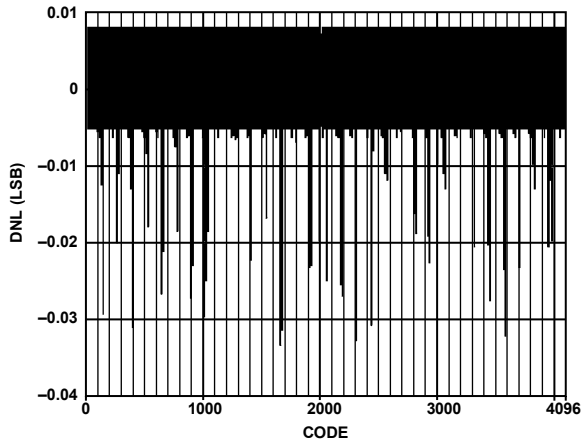
Figure 51. AD9706 Typical Uncalibrated DNL
