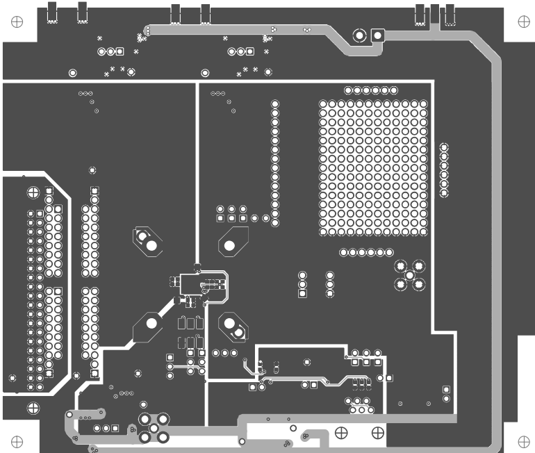
Figure 101. Layer 4—Secondary Side
