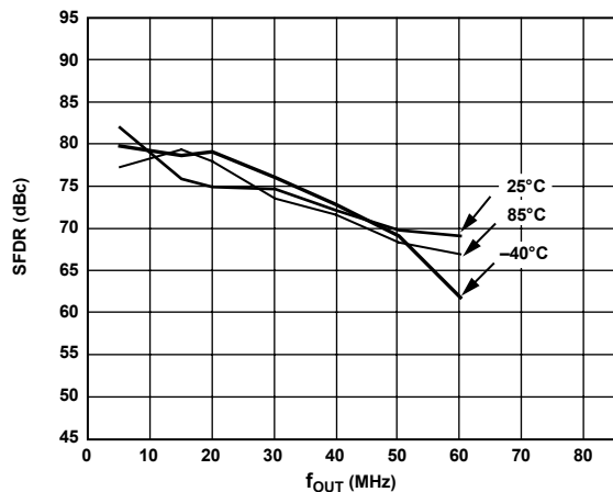
Figure 23. SFDR vs. Temperature @ 175 MSPS
