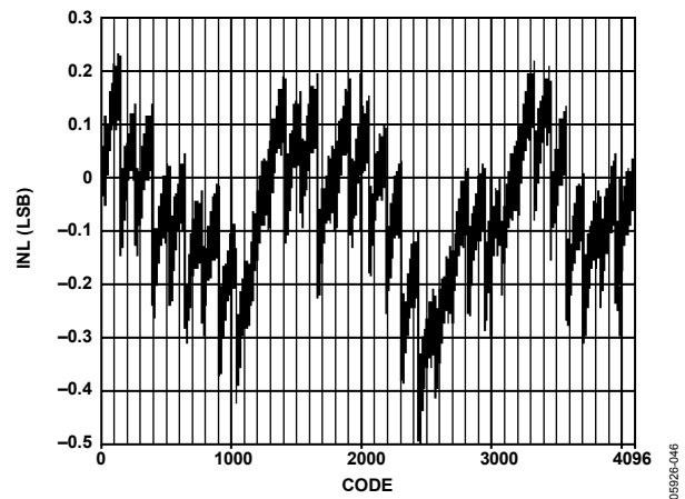
Figure 50. AD9706 Typical Uncalibrated INL
