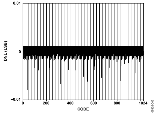
Figure 49. AD9705 Typical Uncalibrated DNL
