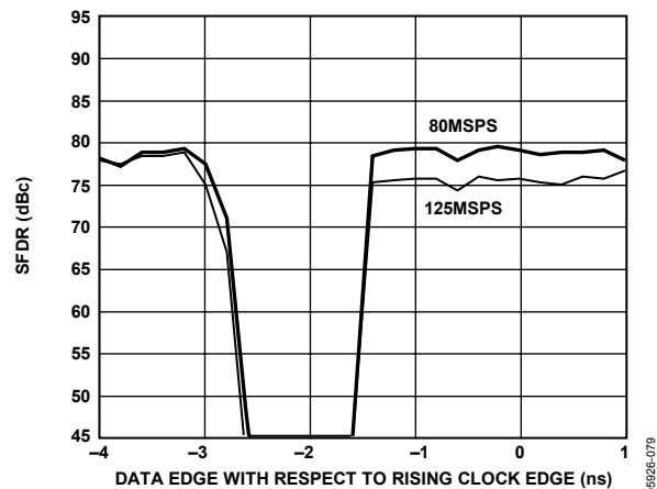
Figure 81. SFDR vs. Clock Placement
