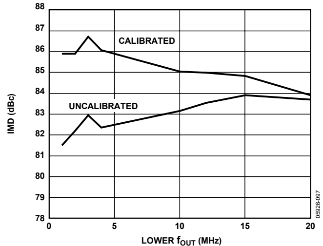
Figure 89. IMD vs. f OUT @ 175 MSPS and I OUTFS = 2 mA
