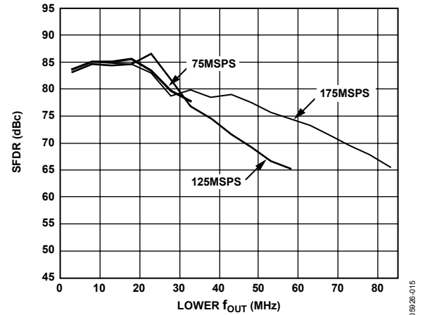
Figure 17. Dual-Tone IMD vs. f_{OUT} @ 0 dBFS
