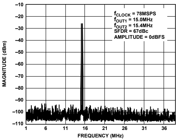
Figure 66. AD9704 Dual-Tone SFDR
