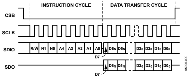
Figure 74. Serial Register Interface Timing, MSB First Read
