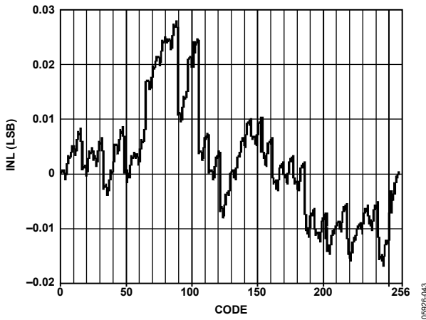
Figure 46. AD9704 Typical Uncalibrated INL
