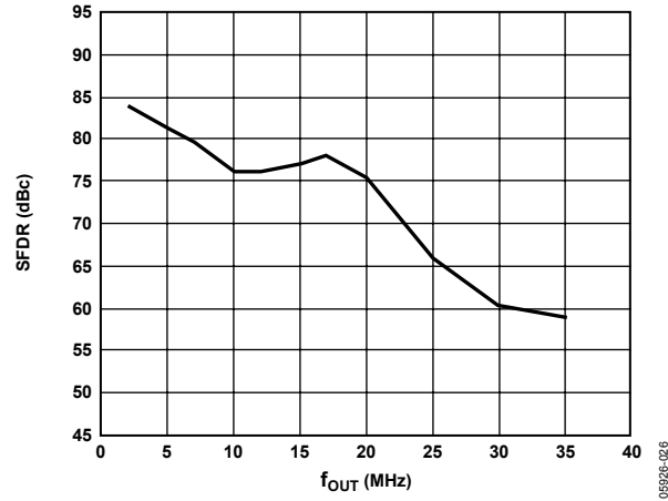
Figure 30. SFDR vs. f_{OUT} @ 80 MSPS
