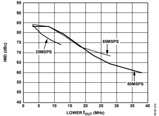
Figure 36. Dual-Tone IMD vs. f_{OUT} @ I_{OUTS} = 2 \text{ mA} and 0 \text{ dBFS}
