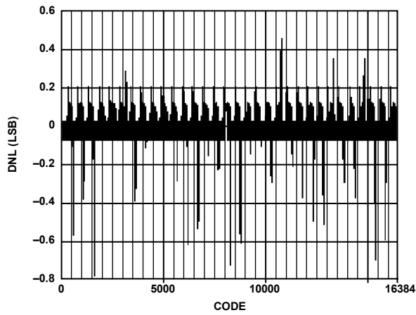
Figure 40. Typical Uncalibrated DNL
