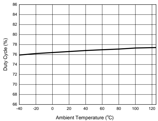
Figure 9. Duty Cycle vs. Ambient Temperature
