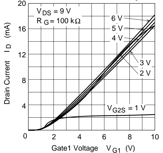
Drain Current vs. Gate1 Voltage
